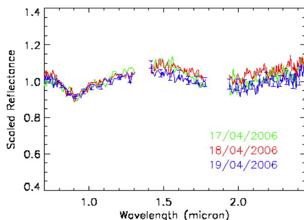
Fig. 4: Karin spectra obtained during three consecutive nights with SpeX (IRTF). The spectra are normalized to unity at 0.8 \mu\text{m} .
