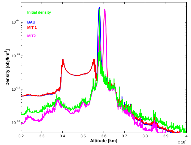
Figure 5. GEO region: initial (2005) and final (2205) spatial density of objects larger than 1 m in the BAU, MIT1 and MIT2 scenarios.
