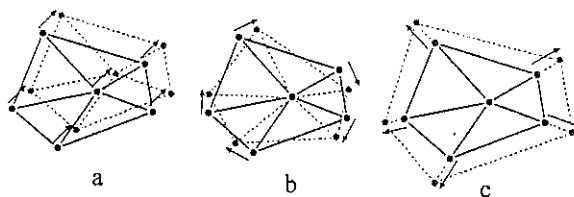
Fig. 6. Even if only translations are computed for each vertex, the combination of all of these transformations may result in a affine transformation of the corresponding target image section.
