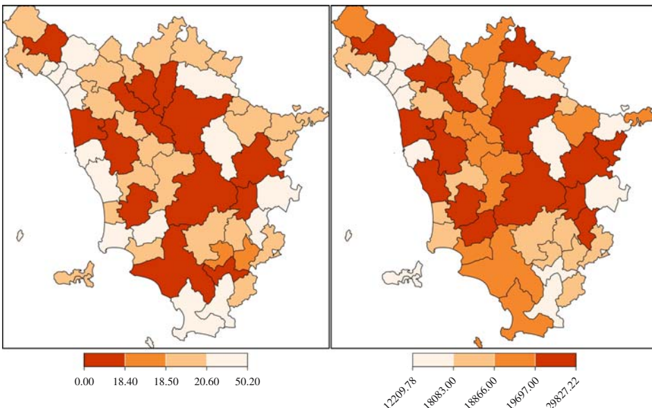
Fig. 2. Estimates of the mean equivalised income in Euros (right) and of the HCR (left) for the Local Labour Systems of Tuscany region. Small area estimates based on EU-SILC 2011 and Mobility Data 2011. Out-of-sample areas are estimated using a synthetic estimator.
