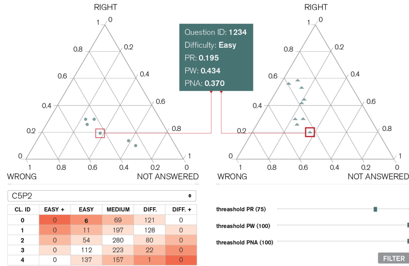
Fig. 6. An example of outlier detection using cluster analysis (left) and visualization-based approach (right).
