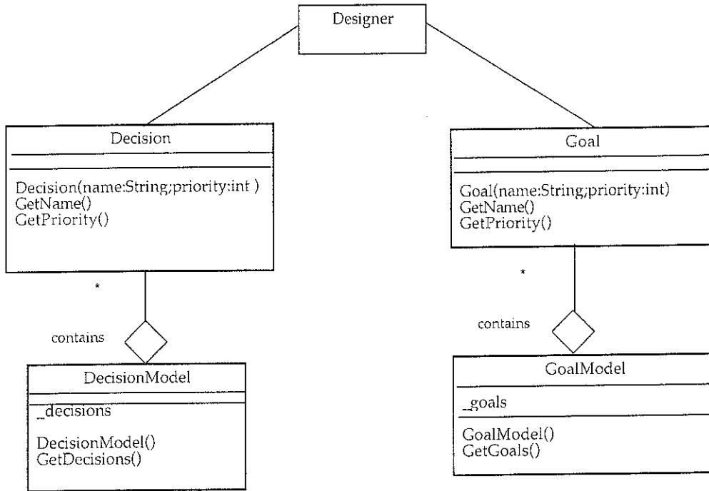
Fig 3: Class diagram of the selected Use case for uci.argo.UserModel
