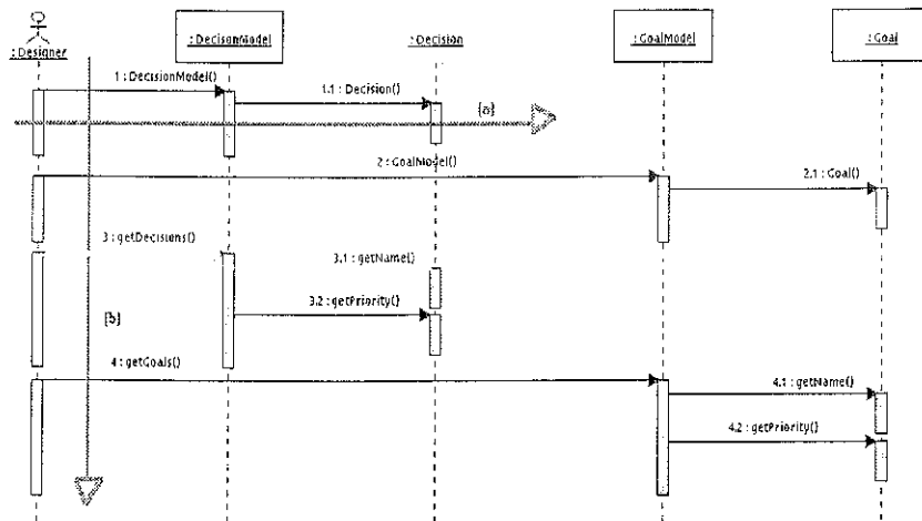
•Sequence diagram of uci.argo.Kernel.USERMODEL
