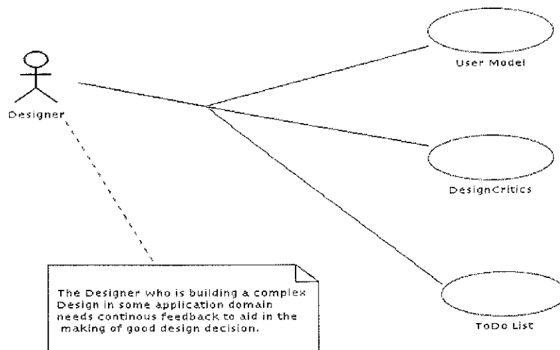
Fig 1: Use Case diagram (of uci.largo.Kernel)
