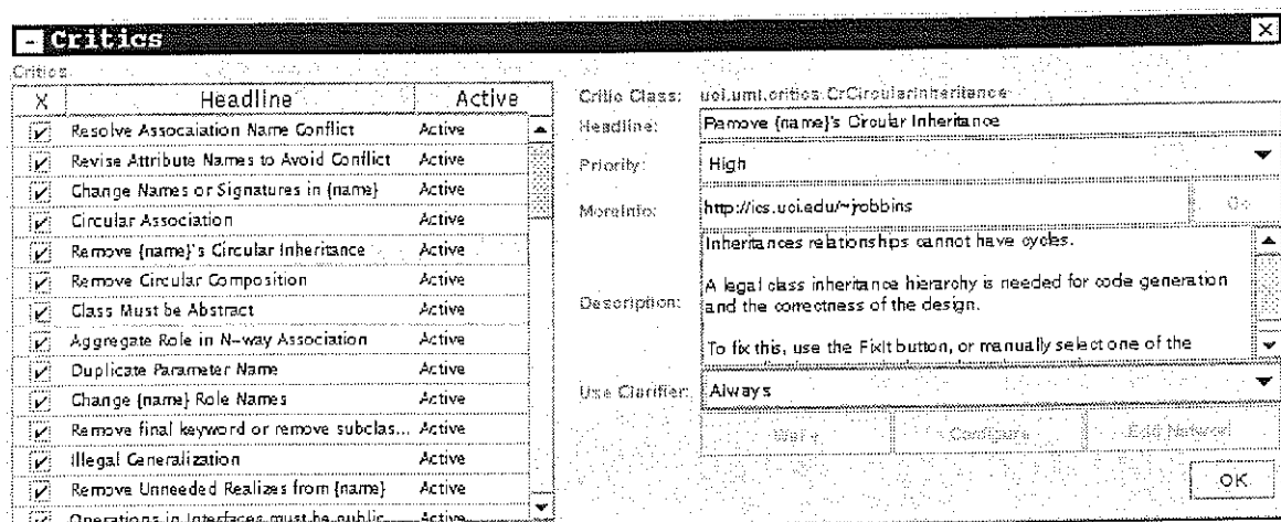
Fig 4: Argo/UML Critic Browse Windows
