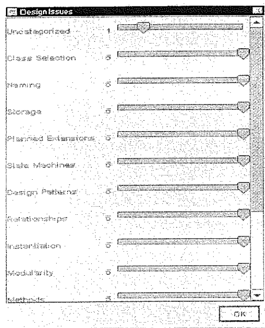
Fig 6: Argo/UML Design Issues Panel and Design Goals Panel
