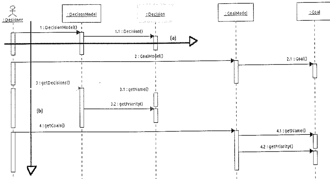
Fig 2: Sequence diagram analysis
