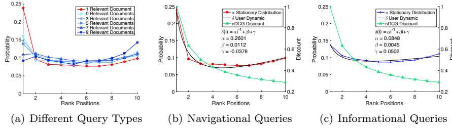
Fig. 1 Stationary distributions for queries retrieving different number of relevant documents (a), and stationary distribution with its fitted curve and DCG discount for navigational (b), and informational queries (c).
