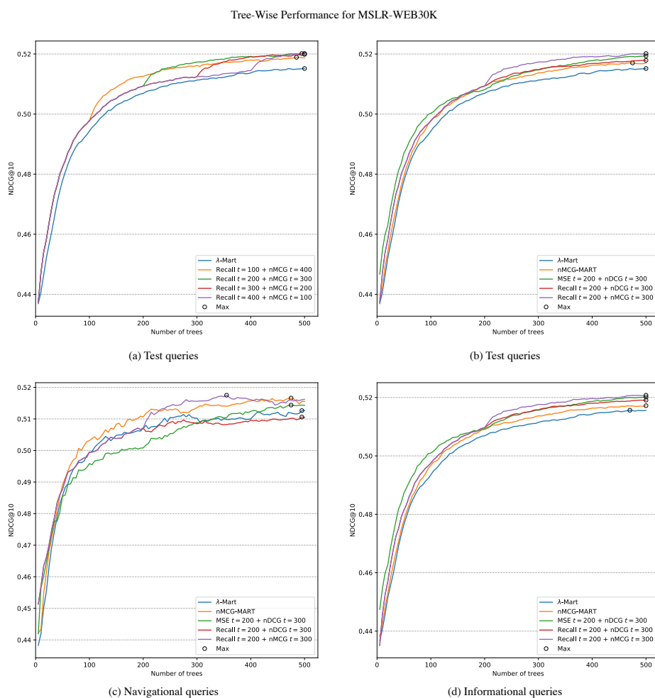
Fig. 2 Comparison of continuation methods approaches trained with nMCG and with different switching points (a) and comparison of different models on test queries (b), just on navigational queries (c) and just on informational queries (d). All the figures refers to MSLR-WEB30K Fold 1 and all the models are evaluated with respect to nDCG@10.
