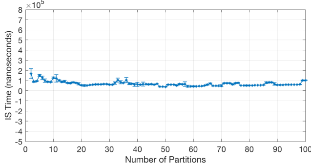
Fig. 3. Importance Sampling time: median and SIQR
