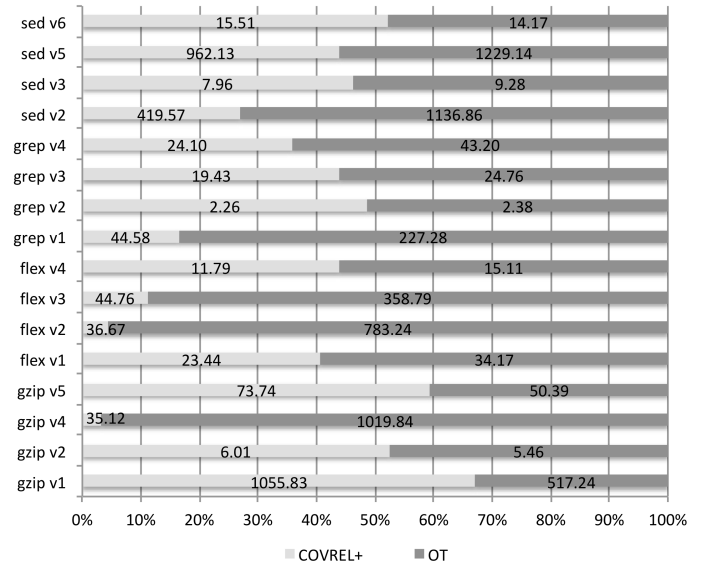
Fig. 9. Test Generation: Additional test cases by subject
