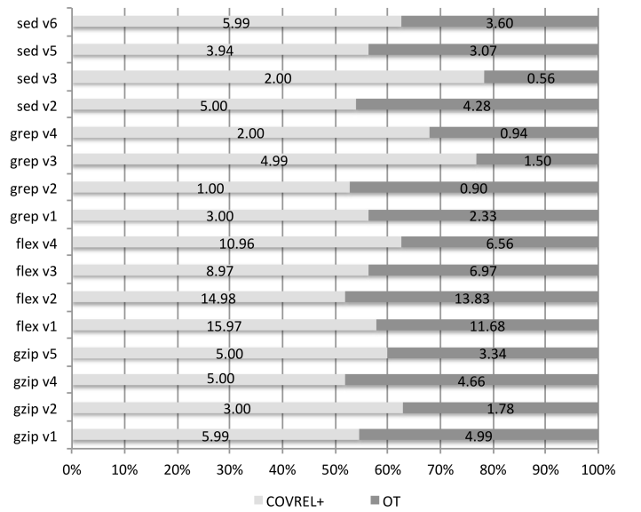
Fig. 11. Test Generation: Percentage and number of faults by subject
