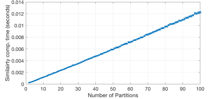
Fig. 5. Similarity computation time: median and SIQR
