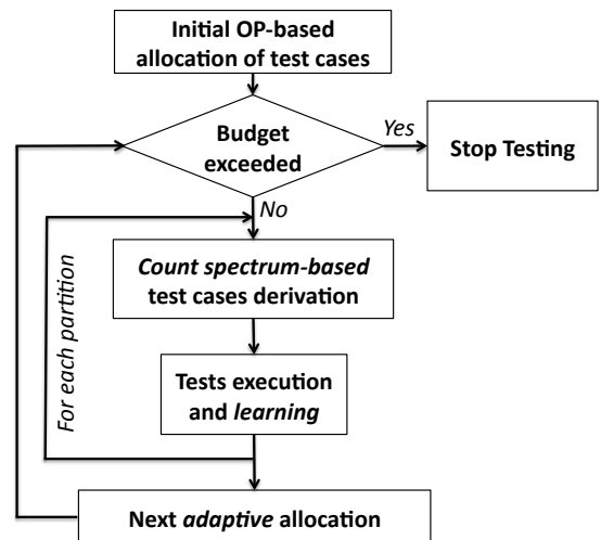
Fig. 1. The covrel+ strategy
