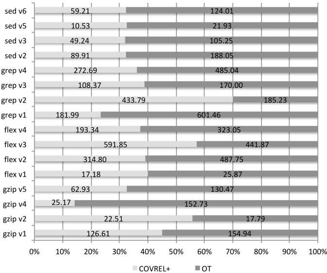
Fig. 7. Test Selection: Additional test cases by subject
