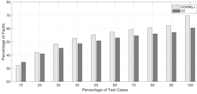
Fig. 12. Test Selection: Faults vs test cases (percentages)
