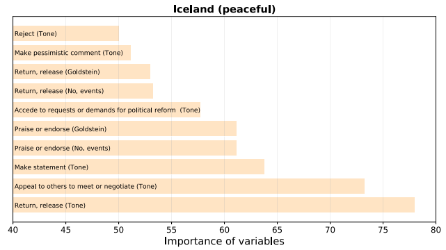
Fig. 5. Important variables for Iceland, a peaceful country. In the parenthesis, we mention the type of variable. The variables are related to releases of people and property, negotiations, public statements, endorsement of people and actions, and political reforms.
