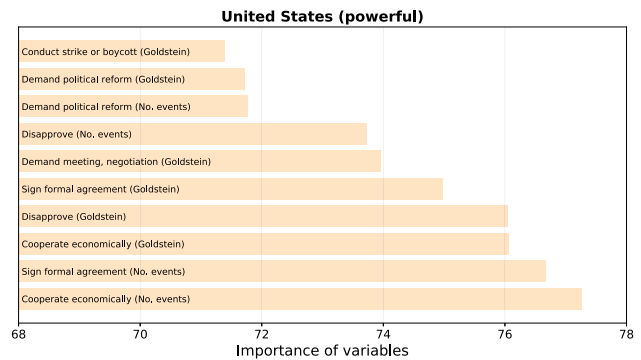
Fig. 6. Important variables for the United States, a powerful country. In the parenthesis, we mention the type of variable. The variables are related to economic and material cooperation, formal agreements and meetings, disapprovals, political reforms, and strikes or boycotts.
