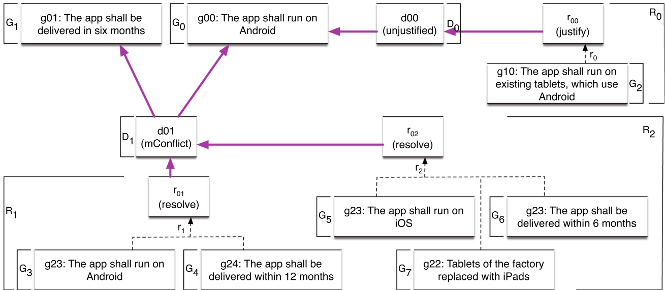
Fig. 5 Example of construction of ASPIC + arguments
