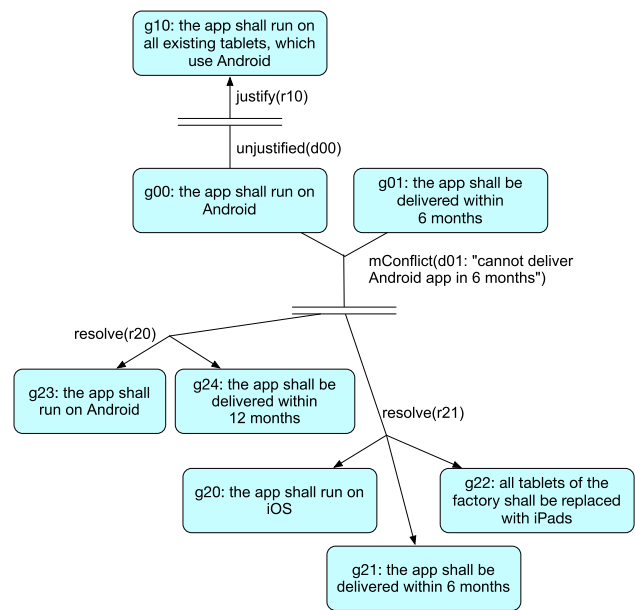
Fig. 4 Refinement graph example
