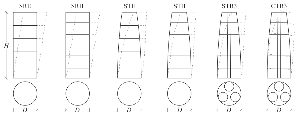
FIGURE 10 Schematics of the models investigated within the parametric analysis. The first letter in the acronym points at the mechanics (Shear type or Cantilever), the second at the building shape (Regular or Tapered), the third at the position of the outriggers (Equally spaced or arranged as per the Bamboo growth model), lastly the number 3 is added for the models that uses a three-bundle setting
