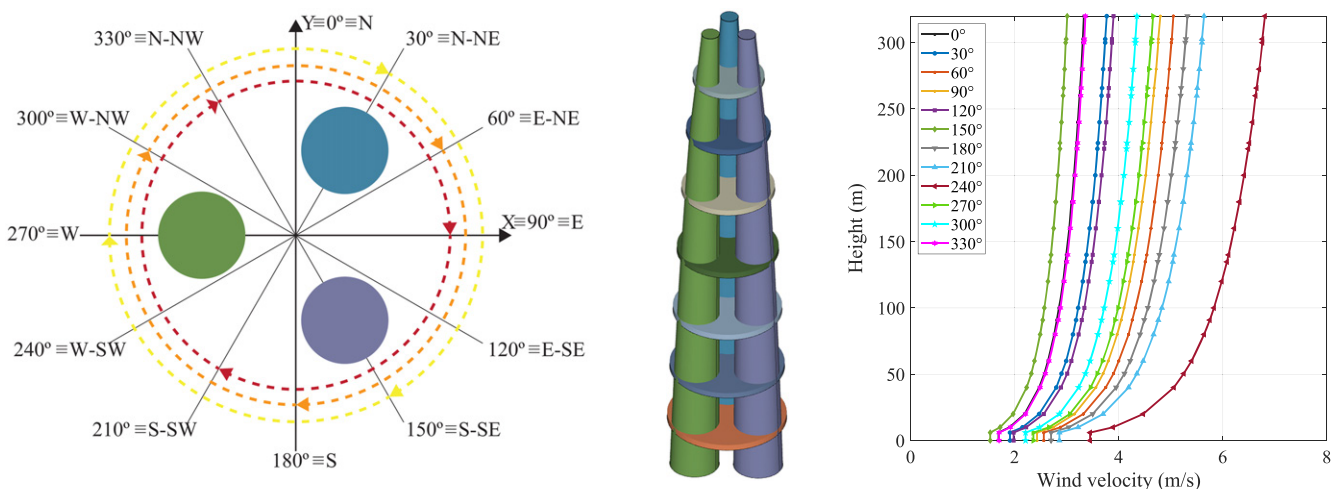
FIGURE 23 3-D CFD analysis: wind rose, model, and adopted wind velocities
