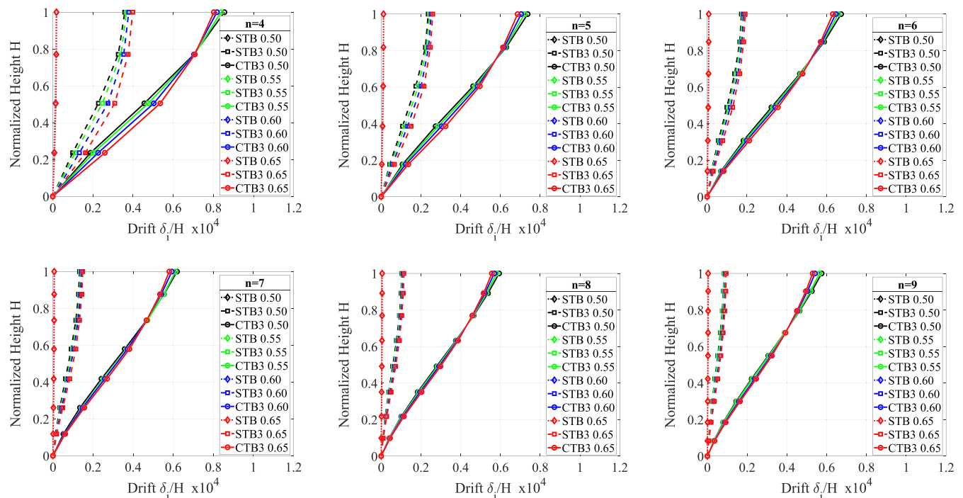
FIGURE 13 Bundling effect for the H = 320 m model (aspect ratio set to 1:4)
