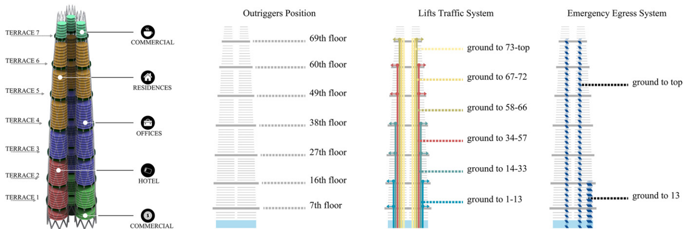
FIGURE 19 Architectural and functional design: functions allocation and vertical circulation
