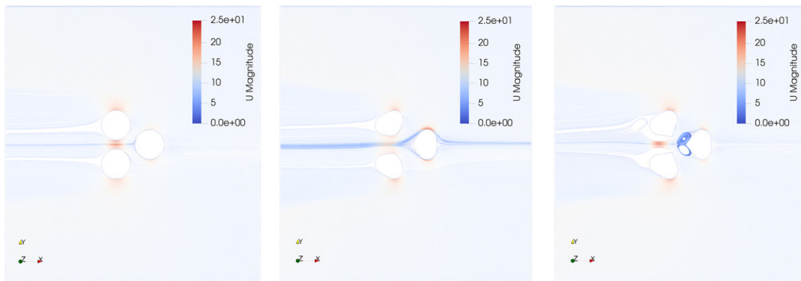
FIGURE 15 2-D CFD results for the cross section shaping ( -X wind): (a) circle; (b) triangle with two corner fillet; and (c) triangle with three corner fillet
