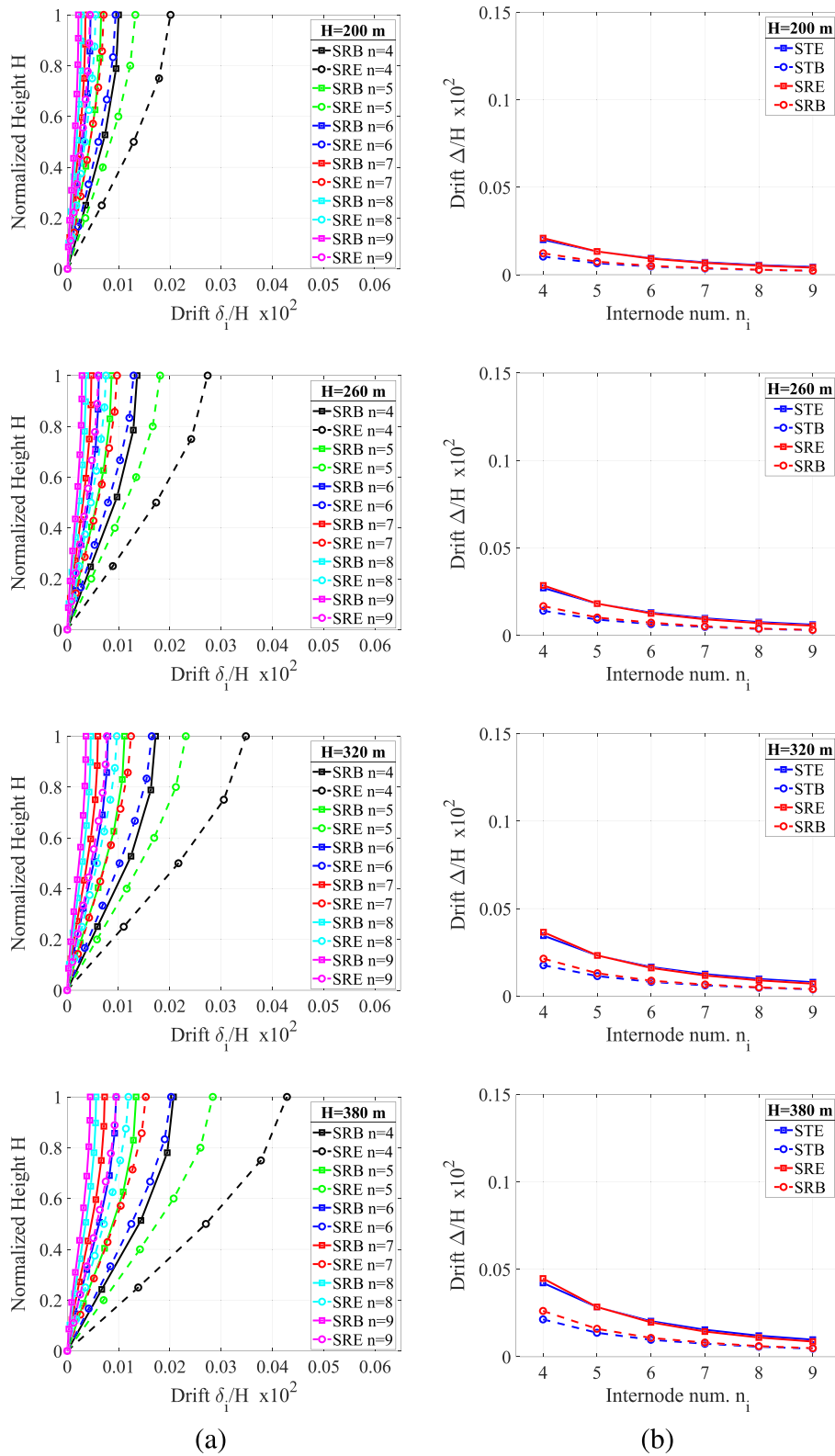
FIGURE 12 Parametric investigation on macroscale parameters and outrigger spacing: (a) qualitative shear-only deformed shape comparison (aspect ratio set on 1:4, bamboo model limit to 0.55 for the SRB); (b) tapering effect (aspect ratio set to 1:4, bamboo model limit to 0.60). The rows denote different heights
