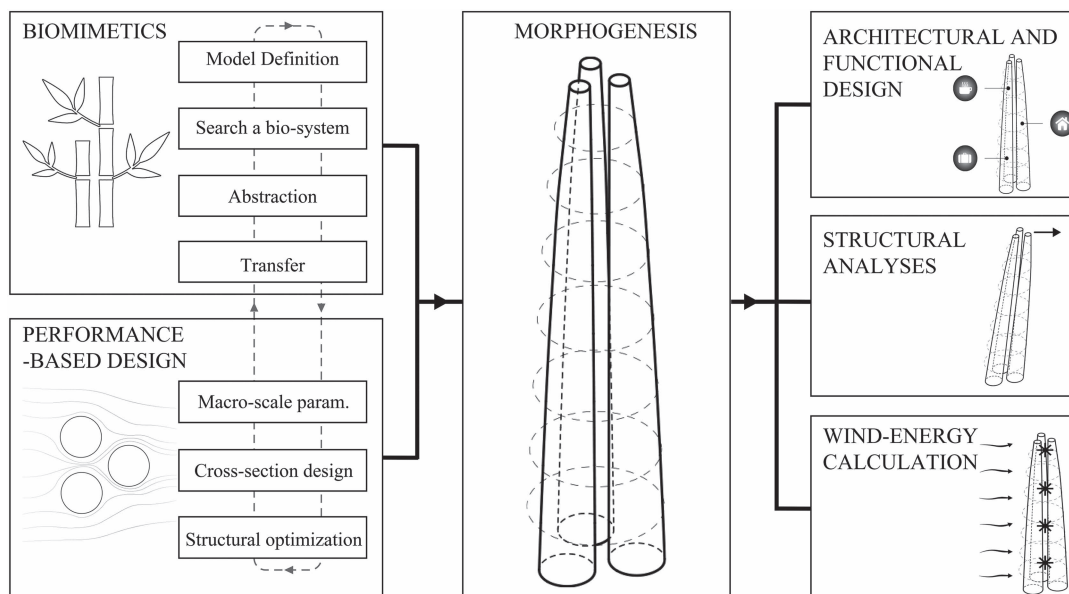
FIGURE 2 Methodological design scheme adopted in this work
