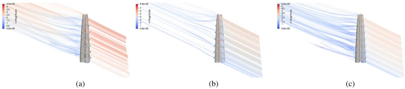
FIGURE 24 Streamline-style representation of the flow in the (a) +X, (b) -X, and (c) Y cases
