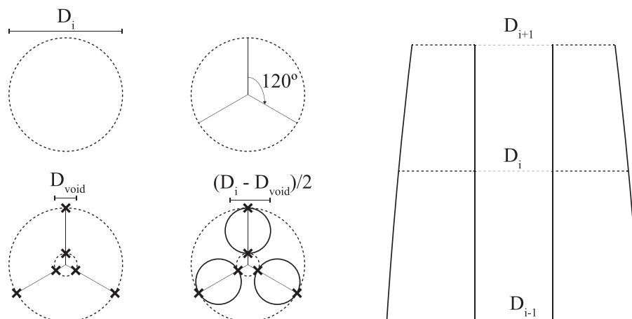
FIGURE 8 Geometry generation of the bundled building within the bamboo model design space
