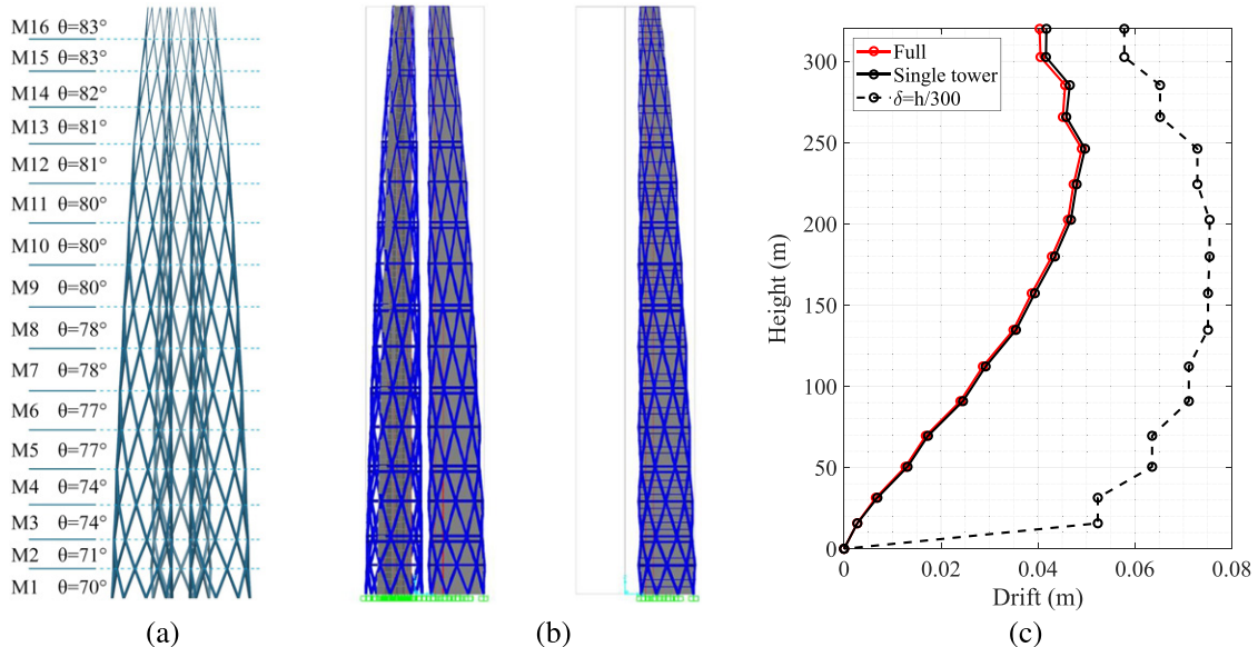
FIGURE 17 Diagrid optimization: (a) angles; (b) full and single-tower simplified models; (c) drift comparison
