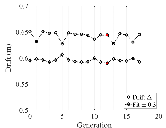
FIGURE 18 Size optimization results obtained by means of Galapagos: total drift \Delta and fitness function variation
