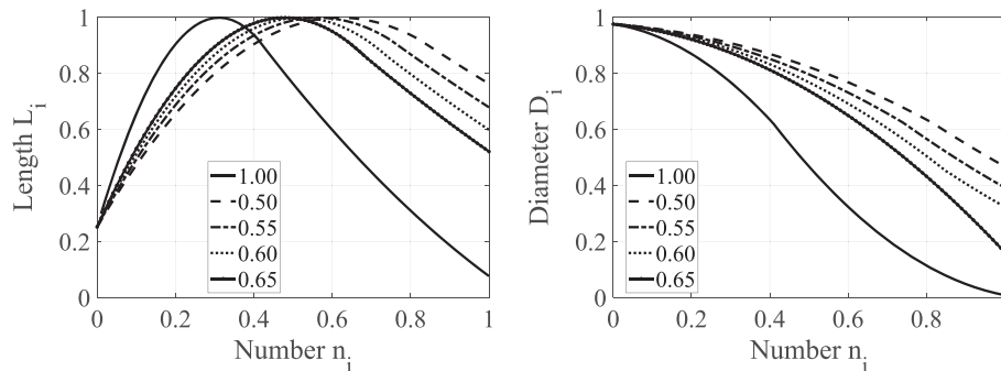
FIGURE 7 Rescaled bamboo functions with different model limits (0.50, 0.55, 0.60, 0.65, 1.00)
