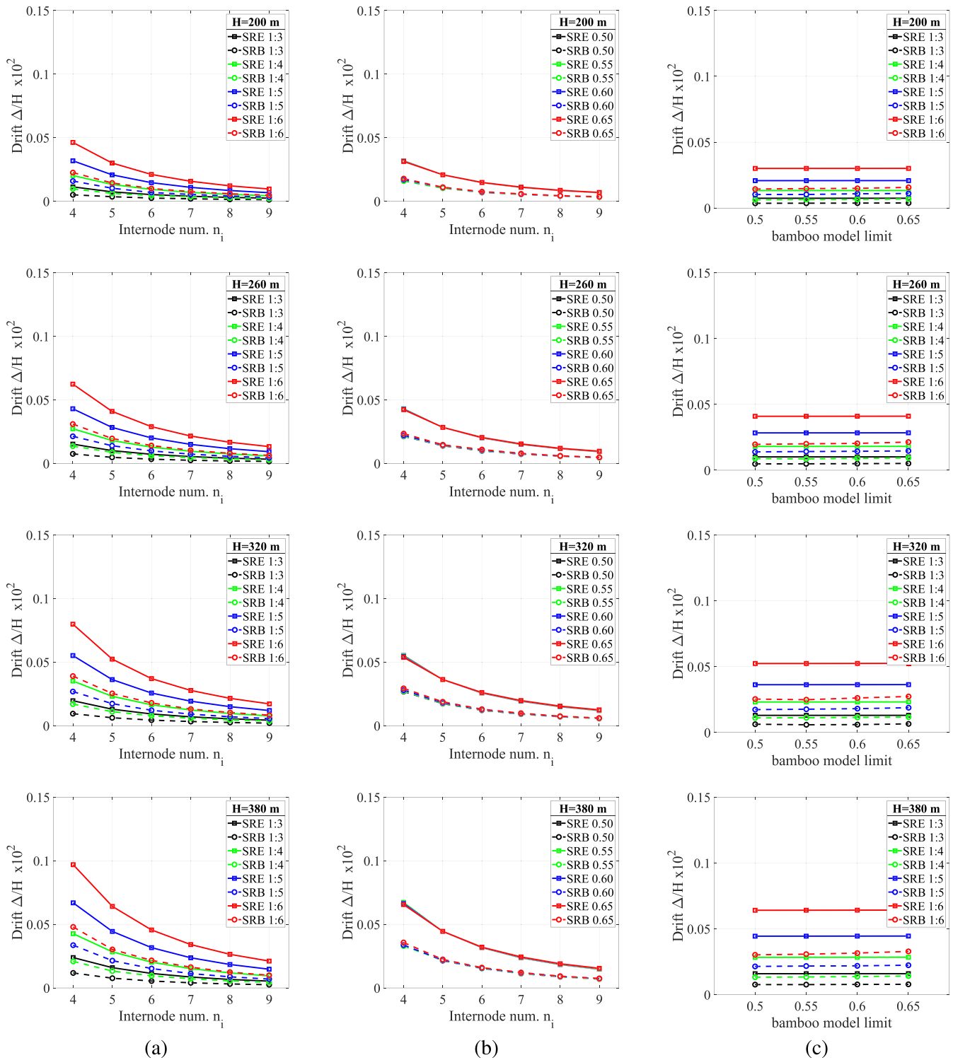
FIGURE 11 Parametric investigation on macroscale parameters and outrigger spacing: (a) aspect ratio (growth model limit set to 0.5); (b) growth model limit (aspect ratio set to 1:5); (c) aspect ratio (number of nodes set to 6). The rows denote different heights
