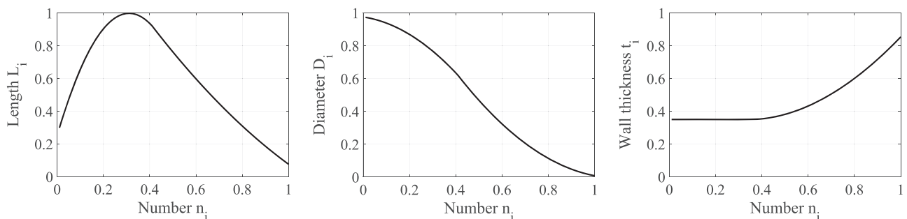
FIGURE 3 Function plots of the bamboo growth pattern as per Equations (1)–(3). The parameter t_i is reported for completeness but has not been used in the present methodology
