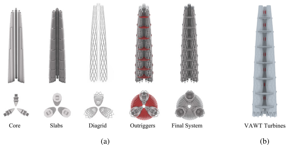
FIGURE 5 Structural system introduced in the present concept (a) and VAWT building integration (b). The figure illustrates the design solution adopted in the case study
