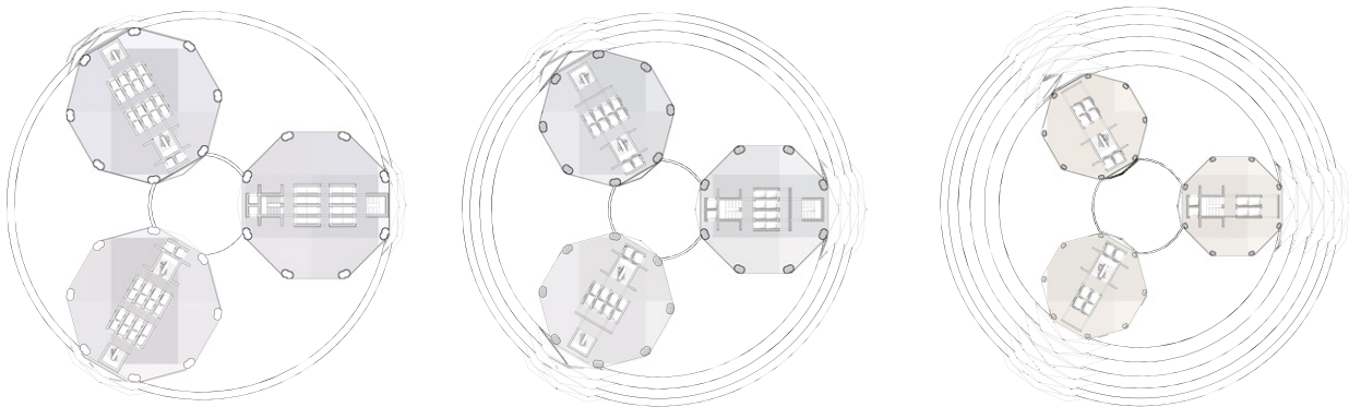
FIGURE 20 Floor plans at level 69.5, 157.2, and 246.2 m (ref. colors to Figure 19)
