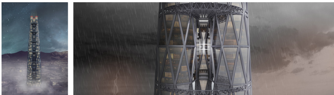
FIGURE 1 Render views of the proposed concept for a bundled tall building applied to a 320-m-tall case study in Pisa: overall view and detail of the vertical axis wind turbine
