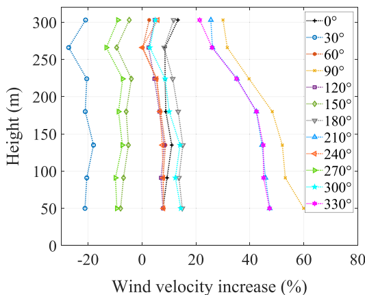
FIGURE 25 Wind velocity variation between the inlet velocity and the average velocity in the VAWT area
