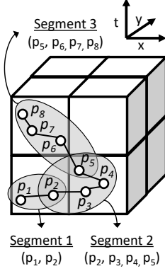
Figure 1: Trajectory segmentation.
