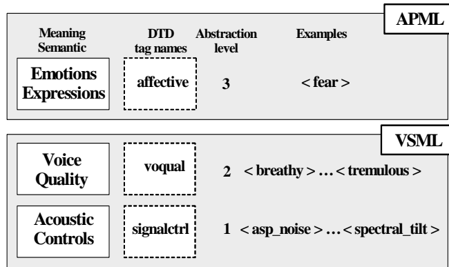
Fig. 4. APML/VSML mark-up language extensions for emotive audio/visual synthesis.
