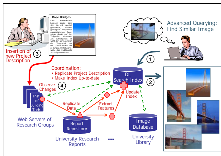
Fig. 1: Management and Coordination of Information Spaces
