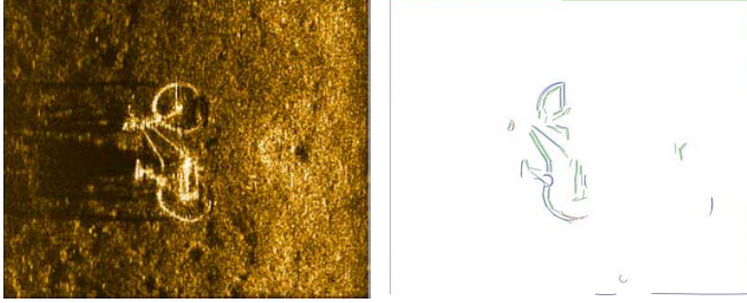
Figure 4: ELSD curve detection result on a sonar map Imagery from jwfishers.com
