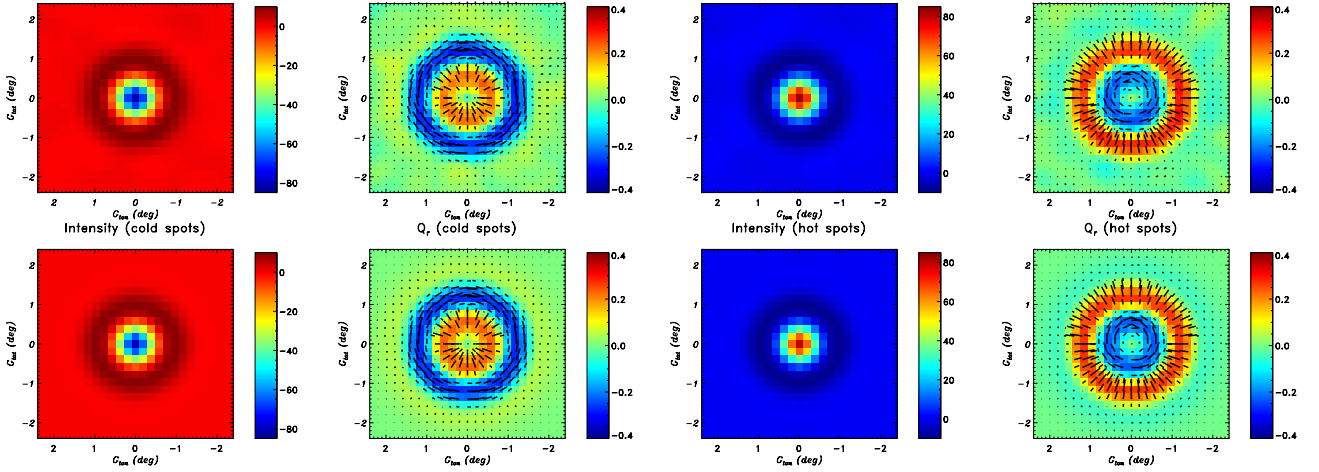
Fig. 27. Stacked maps of the CMB intensity I and polarization Q , at the position of the temperature extrema, at a common resolution of 30 arcmin. Maps are displayed for CMB temperature cold spots (left) and hot spots (right) for the Planck CMB estimates (top row) and for the \Lambda CDM Planck best fit model prediction (bottom row).
