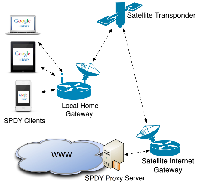
Figure 1. Reference architecture of the adopted tested. The satellite link has been emulated with different values of RTT and packet loss.
