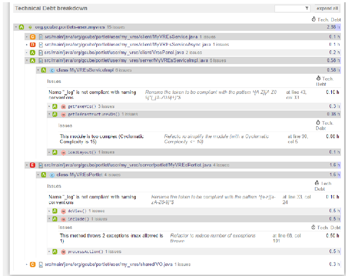
Figure 7: SQALE Report
