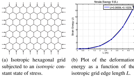
Figure 4: Derivation of \mathbf{U}_d(|\bar{u}|, L) for an isotropic hex-grid subject to an isotropic state of stress.
