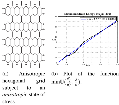
Figure 5: Derivation of the relationship \min \left[ U_a\left(\frac{v_f}{u_f}, \frac{b}{a}\right) \right] for an anisotropic hex-grid subject to an anisotropic state of stress.
