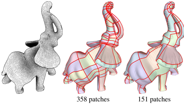
Figure 7: An example of an input cross-field (left), the resulting quad layout (center), and the merged patch decomposition (right) used as the starting point for the greedy optimization process.
