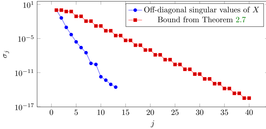
FIG. 5. Off-diagonal singular values in the solution X to (1) where C is a random diagonal matrix and A = B = MM^T with M bidiagonal matrix with ones on the main diagonal and random elements – chosen in (0, 1) – in the subdiagonal. The dimension of the matrices is n \times n with n = 300 . The blue dots represent the most significant singular values of the off-diagonal block X(\frac{n}{2} + 1 : n, 1 : \frac{n}{2}) . The red squares represent the theoretical bound given by Theorem 2.12.
