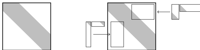
FIG. 3. Graphic description of the quasiseparability of banded matrices; in grey, the non zero entries
