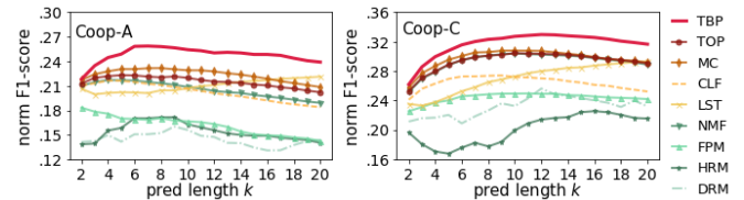
Fig. 7. Normalized F1-score varying predicted basket length k .
