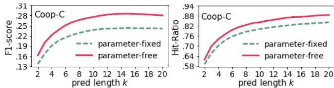
Fig. 5. Next basket prediction performance on Coop-C observing F1-score (left) and Hit-Ratio (right) comparing the parameter-free proposed approach versus the same approach with the parameters fixed.
