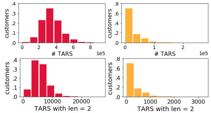
Fig. 4. Number of TARS per customer distribution on Coop-C : parameter-free (left) versus parameter-fixed (right) TARS extraction. The bottom line reports a focus of the distributions of the base TARS, i.e., TARS with length equals to 2.
