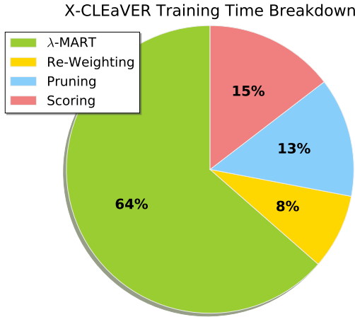
Fig. 6. X-CLEAVER computational cost breakdown. The hyper-parameters adopted are p = 75\% and n = 400 on the Istellla-S dataset.
