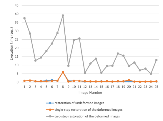
Fig. 9 Plots of the execution times (in seconds) for the 25 images of the database in [23]. Blue line: restoration of the undistorted images; red line: single-step restoration of the distorted images; gray line: two-step restoration of the distorted images.
