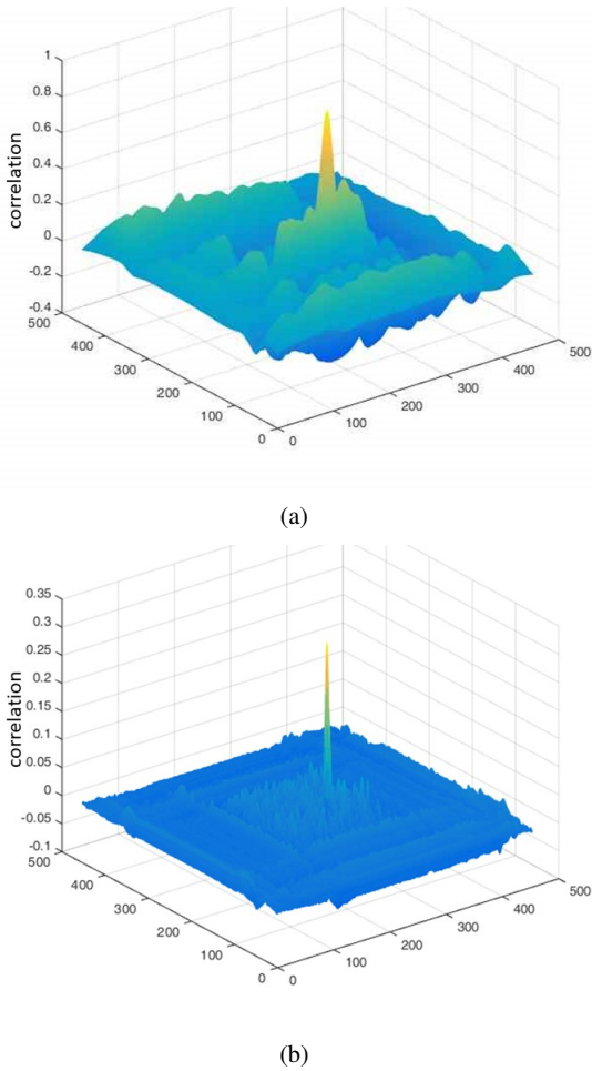
Fig. 2 Correlation matrix computed on the intensities (a) and on the gradients (b).
