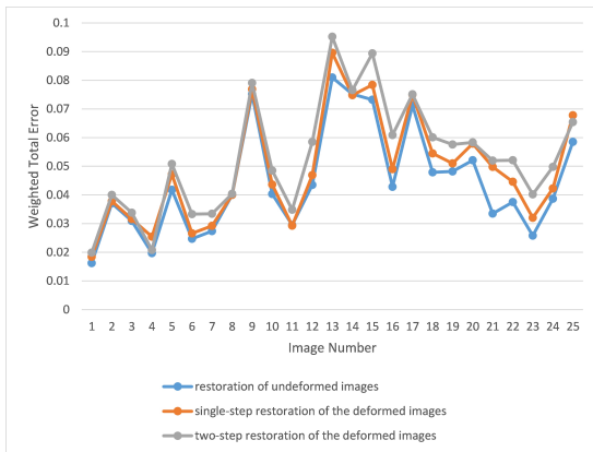
Fig. 8 Plots of the Weighted Total Errors for the 25 images of the database in [23]. Blue line: restoration of the undistorted images; red line: single-step restoration of the distorted images; gray line: two-step restoration of the distorted images.
