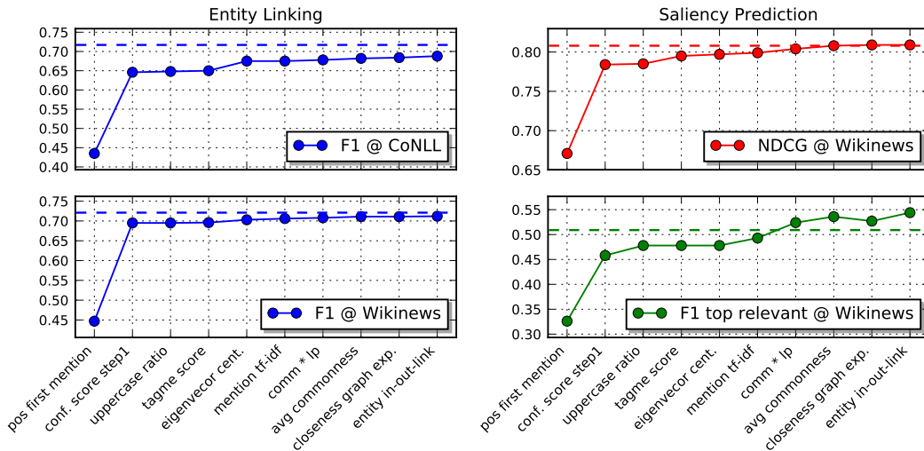
FIGURE 2. Incremental performance on step 2 using top k features.
