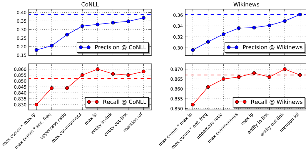
FIGURE 1. Incremental performance on step 1 using top k features.
