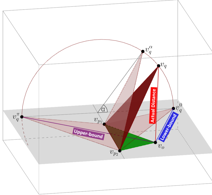
Figure 1: Example four-point based projection. Two reference objects p_1, p_2 and two data objects o, q are first isometrically embedded in 3D Euclidean space. The mapped points are indicated with v_{p_1}, v_{p_2}, v_o, v_q in the graph. By rotating v_q around the edge \overline{v_{p_1}v_{p_2}} we obtain the points v_q^\alpha where 0 \leq \alpha \leq \pi is the angle formed with the triangle \Delta v_{p_1}v_{p_2}v_o . A planar projection is obtained by setting \alpha = 0 or \alpha = \pi . The euclidean distances \ell_2(v_q^0, v_o) and \ell_2(v_q^\pi, v_o) are respectively a lower bound and an upper bound for the actual distance d(o, q) .
