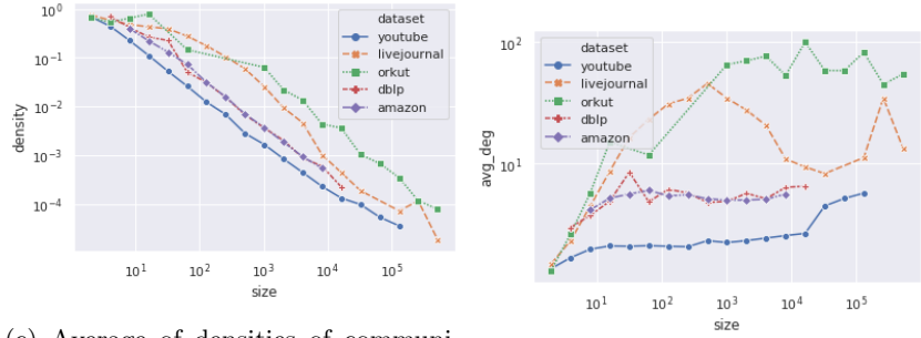
(c) Average of densities of communities, communities discovered by the Louvain algorithm (d) Average of internal mean degree of communities, communities discovered by the Louvain algorithm
