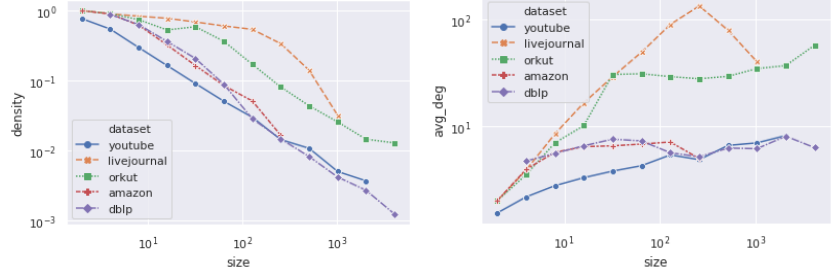
(a) Average of densities of communities, Ground Truth Communities (b) Average of internal mean degree of communities, communities discovered by the Louvain algorithm
