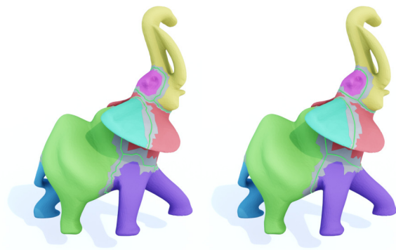
Fig. 6. Boundary seams smoothing. Left: the surface seams polyline (green), derived from the DHF partitioning, can freely move within a tolerance region (gray) while preserving DHF-accessibility of the surface regions it delimits. Right: the same polyline is smoothed using the tolerance region as smoothing domain.
