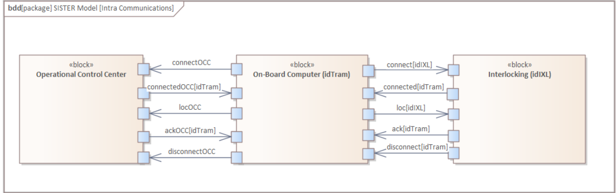
Fig. 3. Intra-Communications diagram
