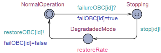
Fig. 13. The OBC_Mitigation automaton
