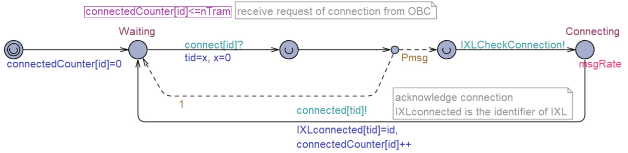
Fig. 16. The IXL_Connect automaton
