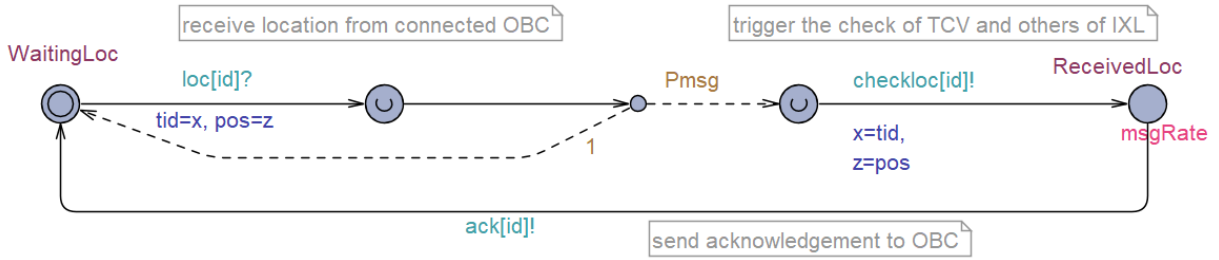
Fig. 17. The IXL_ReceivePos automaton
