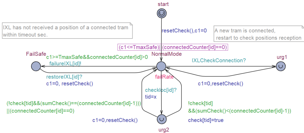
Fig. 18. The IXL_Tmaxsafe_Supervision automaton
