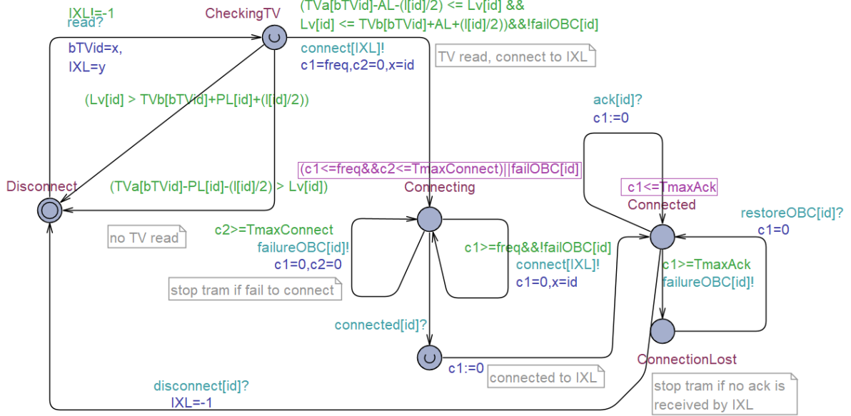
Fig. 14. The OBC_IXLConnectionSupervision automaton.
