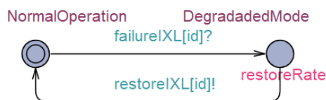
Fig. 20. The IXL_Mitigation automaton
