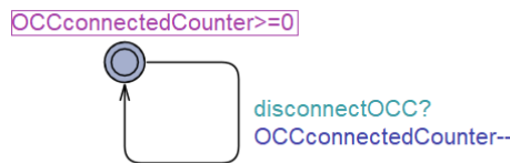
Fig. 6. The OCC_Disconnect automaton
