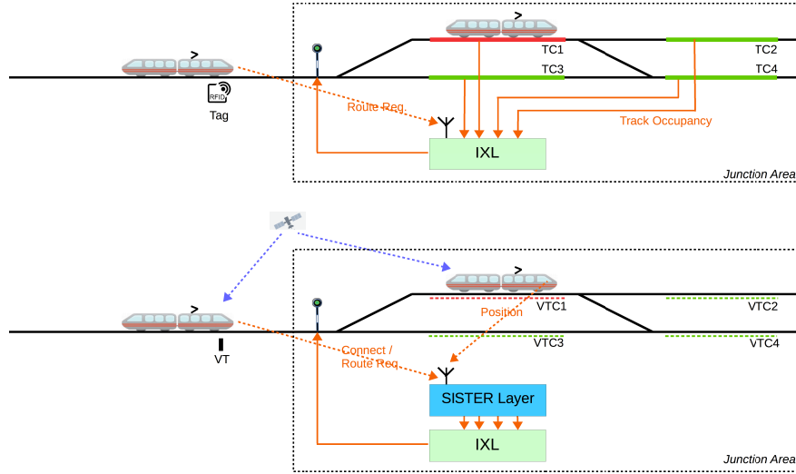
Fig. 1. Substituting track circuits with satellite positioning
