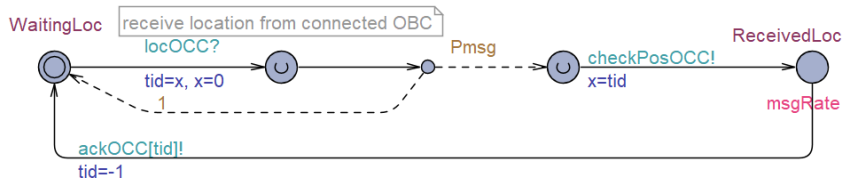
Fig. 5. The OCC_ReceivePos automaton
