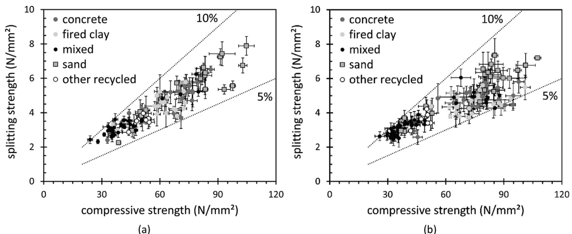
Fig. 12. Splitting versus compressive strength at 7 days (a) and 28 days (b). Error bars represent \pm 1 standard deviation.
