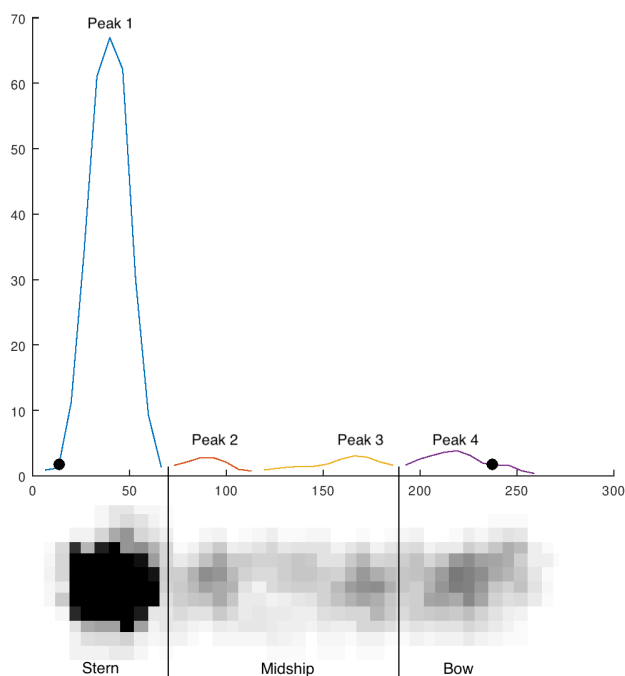
FIGURE 8. OSIRIS-FO: Scattering profile of a bulk carrier ship as estimated by the new feature extractor.
