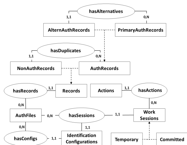
Figure 3 Conceptual data model
