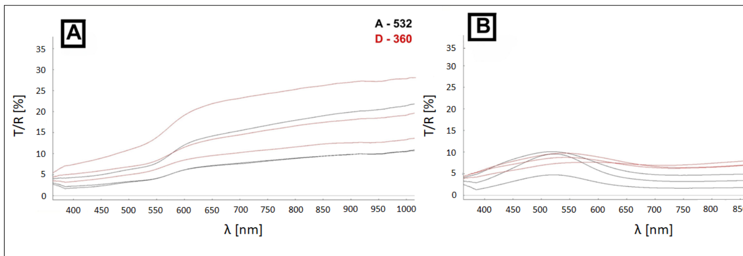
Figure 4. FORS spectra acquired on three different areas of the patina surface: (A) A-532, D-360;(B) B-783, C-1047. (T/R = Transmittance/Reflectance; λ = wavelength).
