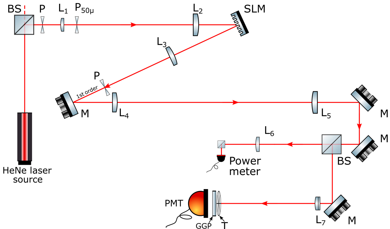
Fig. 1. Light from a HeNe laser at 633 nm is polarized by a polarizing beam splitter (PBS), then spatially filtered and expanded to fill the aperture of an SLM using an aperture (P), a 50-mm focal length lens ( L_1 ), precision pinhole ( P_{50\mu} ), and 400-mm lens ( L_2 ). The SLM displays a superposition of the 6-needle phase masks and a carrier diffraction grating. The SLM is optimized to project the majority of the modulated light into the first diffraction order, which is selected using a 250-mm lens ( L_3 ) and aperture (P) placed in the Fourier plane of the SLM. This light is propagated into the far field through a combination of lenses (250-mm focal length lens ( L_4 ) and 400-mm focal length lens ( L_5 )). The beam is propagated into 2 separate arms using a beam splitter (BS). One arm uses a power meter to measure the laser power and the second arm consists of the target (T) in front of a ground glass plate (GGP). The photomultiplier tube (PMT) measures the transmitted light after interaction with the target. Author figure was adopted from Kallepalli et al. [30].
