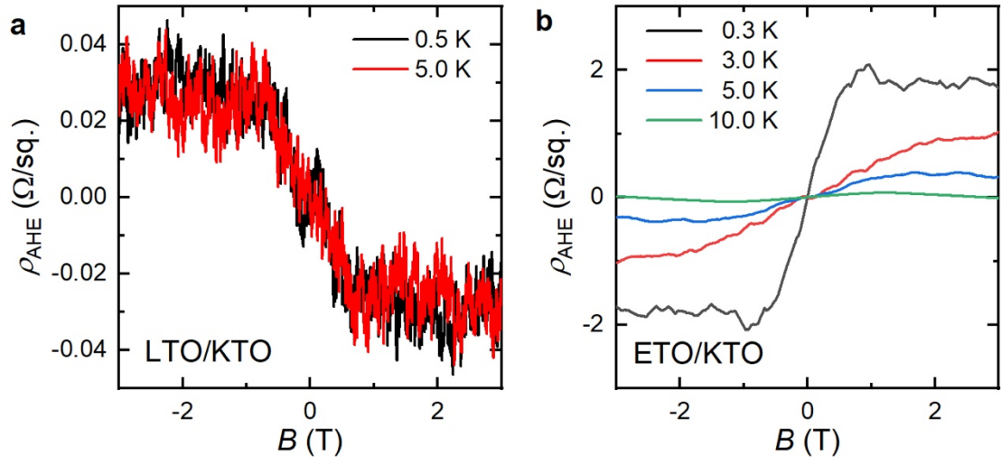
Supplementary Figure 5 Anomalous Hall resistivity for the heterostructures of LTO/KTO (a) and ETO/KTO (b) grown by PLD.
