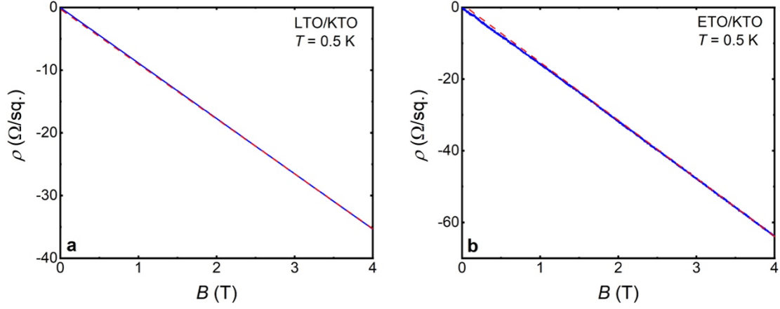
Supplementary Figure 1 Hall resistivity for the sample of LTO/KTO (a) and ETO/KTO (b) grown by MBE.
