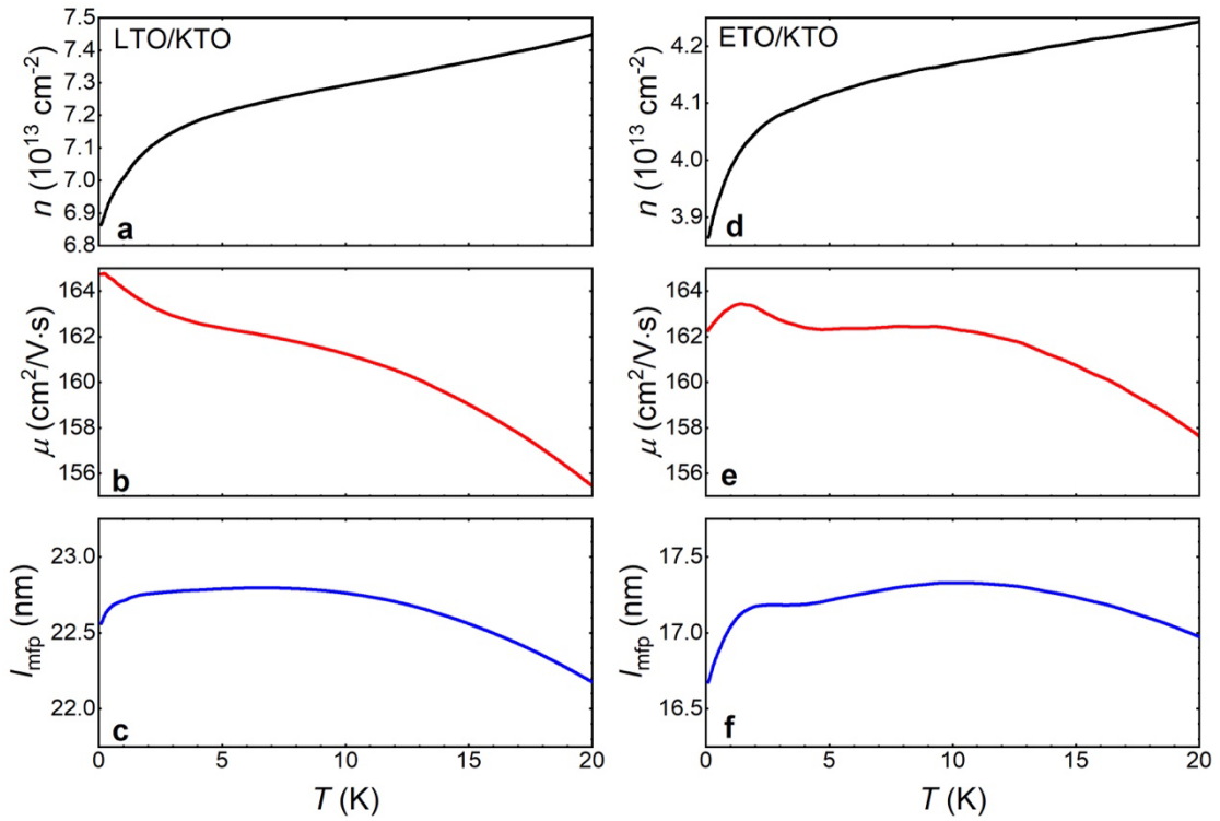
Supplementary Figure 2 Carrier density and mobility of 2DEGs in the sample of LTO/KTO (a & b) and ETO/KTO (d & e) grown by MBE. Mean free paths calculated by Equation S1 based on the carrier densities and mobilities are plotted for the sample of LTO/KTO in (c) and for the sample of ETO/KTO in (f).
