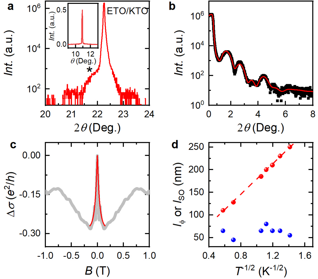
Supplementary Figure 4 Structural characterizations and transport properties of the ETO/KTO heterostructures prepared using PLD technique. (a) XRD scan with the star symbol indicating the (001) peak of ETO. The inset exhibits the rocking curve of the sample. (b) XRR data with red curve a proper fit. (c) Magnetoconductance at 0.5 K with a fitting based on the ILP model in red curve. (d) The extracted lengths l_\phi (red) and l_{so} (blue) with the red dashed line a linear fit.
