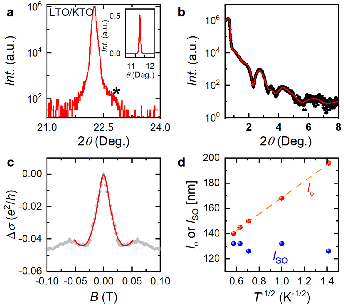
Supplementary Figure 3 Structural characterizations and transport properties of the LTO/KTO heterostructures prepared using PLD technique. (a) XRD scan with the star symbol indicating the (001) peak of LTO. The inset exhibits the rocking curve of the sample. (b) XRR data with red curve a proper fit. (c) Magnetoconductance at 0.5 K with a fitting based on the ILP model in red curve. (d) The extracted lengths l_\phi (red) and l_{so} (blue) with the red dashed line a linear fit.
