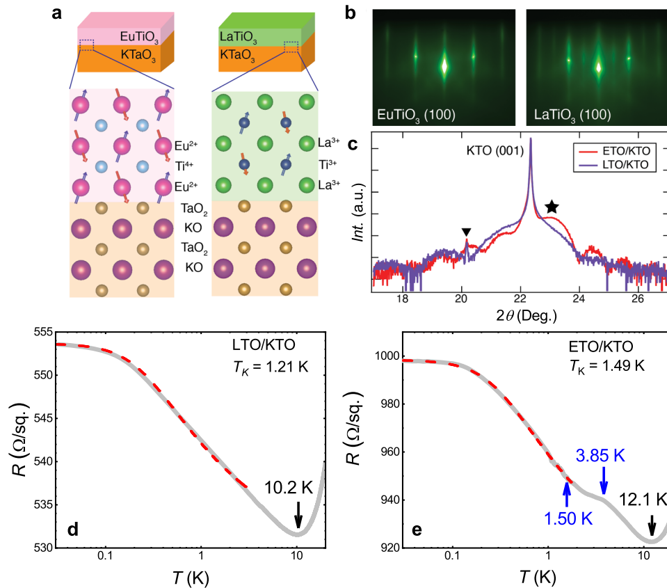
Fig. 1 Structural characterizations and temperature dependence of resistivity for heterostructures of ETO/KTO and LTO/KTO. a Schematic picture of ETO/KTO (left) and LTO/KTO (right) heterostructures and their atomic and antiferromagnetic spin structures (below). The size of spins on the Eu 2+ and Ti 3+ indicates the relative magnitude of magnetic moments ( 7\mu_B/\text{Eu} and 0.5\mu_B/\text{Ti} ). b In-situ reflection high-energy electron diffraction (RHEED) intensity picture of ETO and LTO after 10 u.c. growth. c XRD scan of 20 u.c. ETO/KTO (red) and 10 u.c. LTO/KTO (purple). The symbol ★ and ▼ indicate the (001) peak of ETO and carbon paste defect, respectively. Temperature dependence of resistivity is plotted in (d) for LTO/KTO and in (e) for ETO/KTO.
