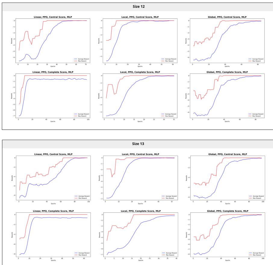
Fig. 6 PPO training performance for graph sizes 12 and 13. Each block shows average and maximum rewards over training epochs. Columns represent the three environments ( Linear , Local , Global ), and rows compare the two reward functions (central vs. complete)
