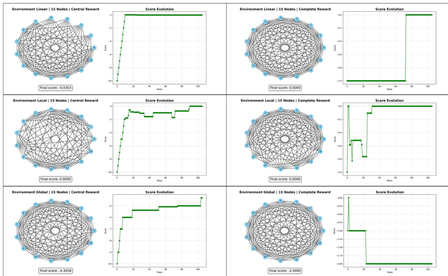
Fig. 11 Best graphs obtained by trained PPO agents for each environment and reward function (15 nodes)
