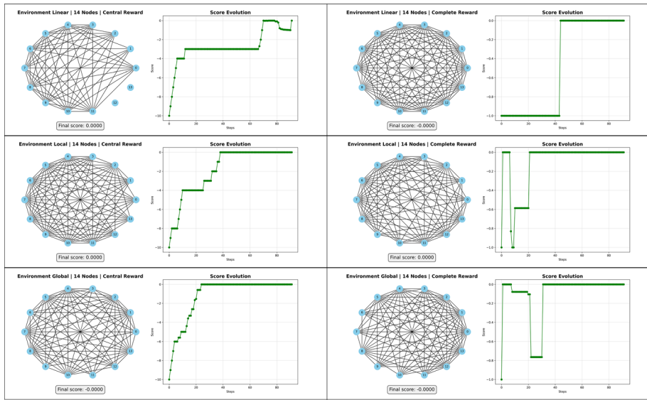
Fig. 10 Best graphs obtained by trained PPO agents for each environment and reward function (14 nodes)
