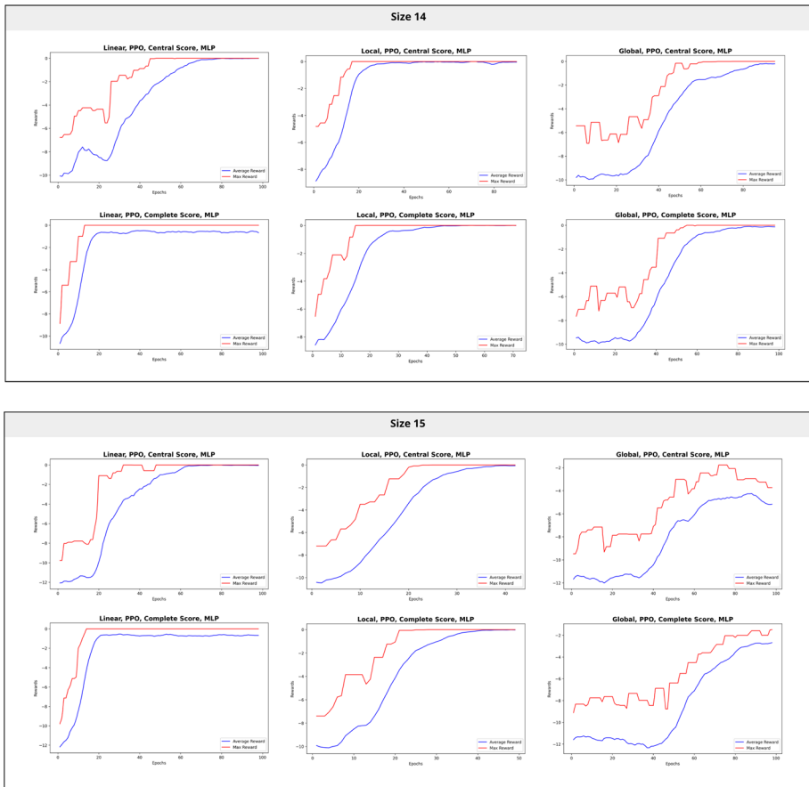
Fig. 7 PPO training performance for graph sizes 14 and 15
