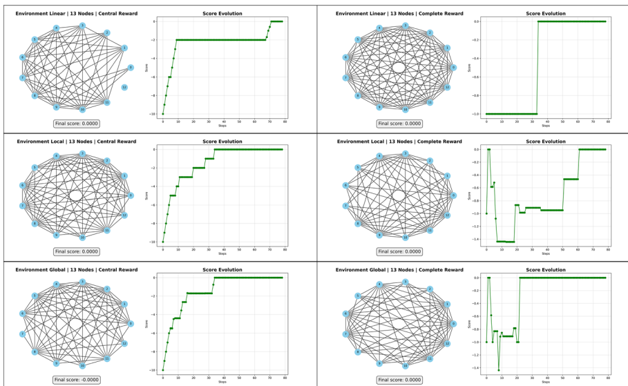
Fig. 9 Best graphs obtained by trained PPO agents for each environment and reward function (13 nodes)
