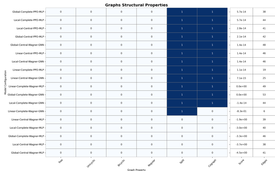
Fig. 4 Plot showing the presence (1) or absence (0) of structural properties across best graph configurations for 11 nodes. Each row corresponds to a specific model configuration (environment, reward function, algorithm, and network type). The properties include being a Tree, Unicyclic, Bicyclic, Regular, Split, or Cograph. To the right of the structural heatmap, the numerical values of the final score and the number of edges are displayed. Configurations are approximately sorted in descending order, as values of order 1e-14 or smaller may result from numerical errors
