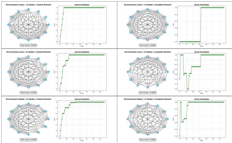
Fig. 8 Best-performing graphs (12 nodes) generated by trained PPO agents with MLP policy, along with score evolution over the episode. Rows correspond to environments ( Linear , Local , Global ); columns to reward functions (central vs. complete)
