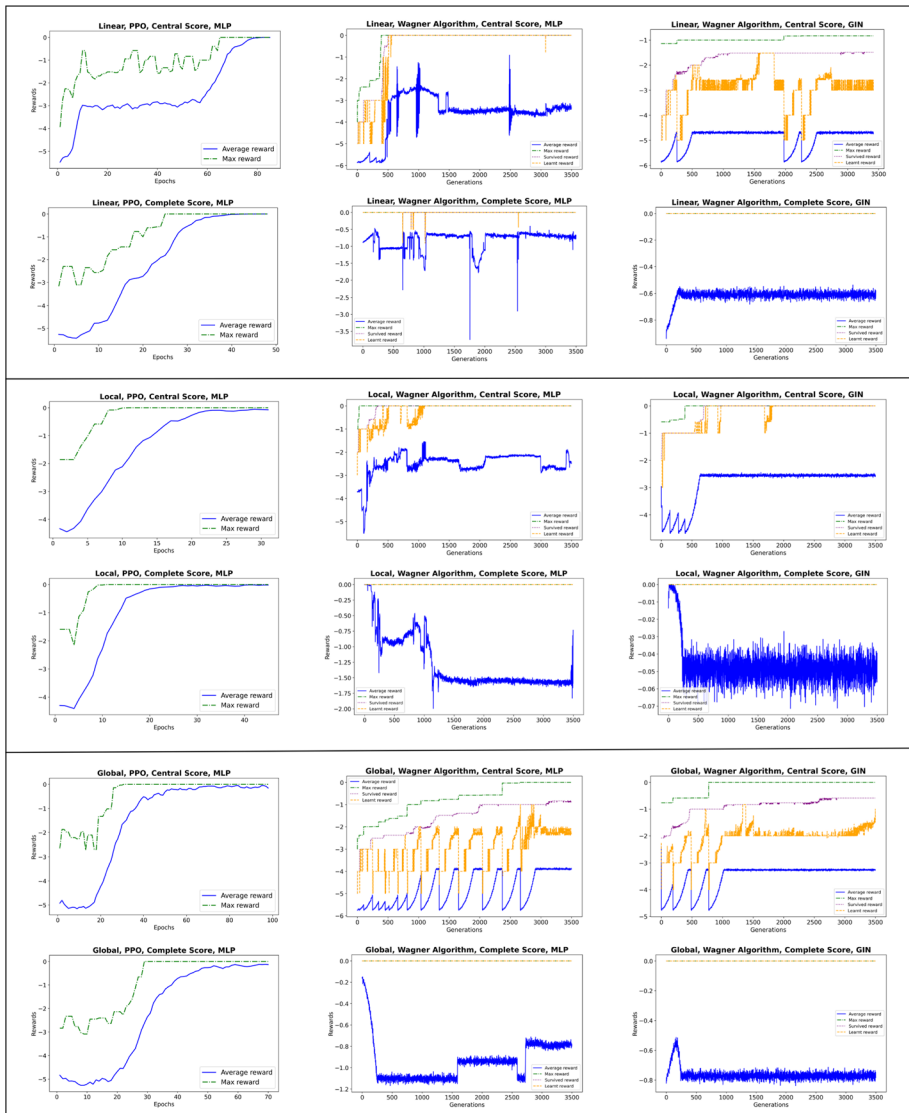
Fig. 3 Comparison of training performance across architectures, reward functions, and environments for graphs with 11 nodes. Each pair of rows represents a different environment ( Linear , Local , Global ), comparing central (top) and complete (bottom) rewards. Columns show results for PPO with MLP (left), and Wagner with MLP (center) or GIN (right). PPO reports average and max rewards per epoch; Wagner includes additional metrics such as survived and learnt rewards
