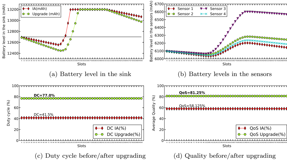
Fig. 4: Case 1: Battery levels in the sink and in the sensors after upgrading (above); duty cycle and quality (below) after the initial assigning (IA) of the most efficient plan and after upgrading.
