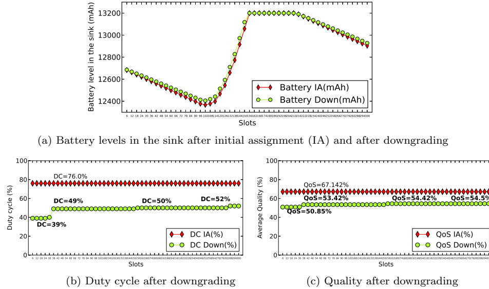
Fig. 7: Case 2: Battery level in the sink (above) and duty cycle and quality (below) after the initial assigning (IA) of the most efficient plan and after downgrading.
