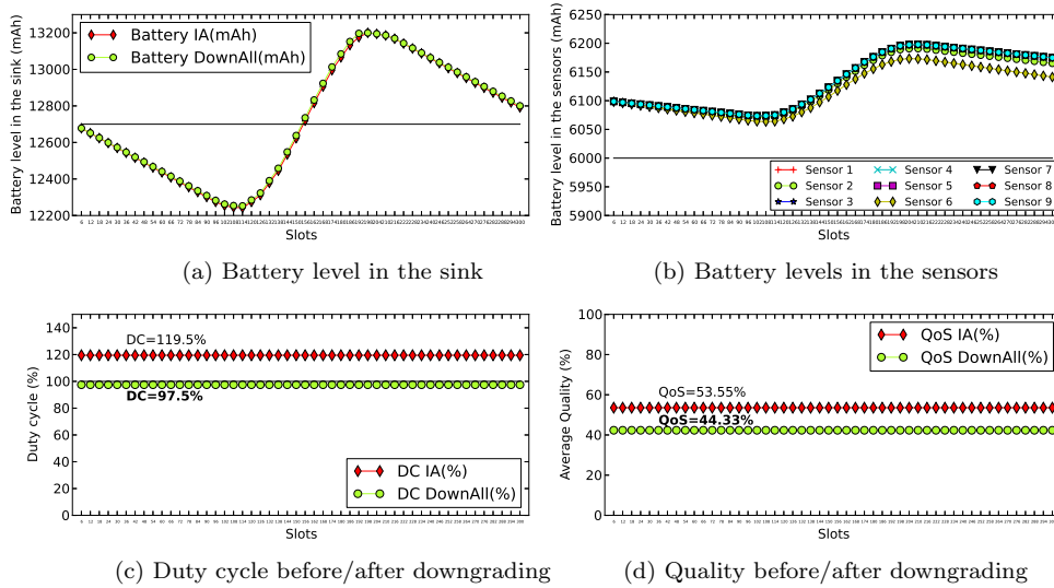
Fig. 8: Case 3: Battery levels in the sink and in the sensors after downgrading (above); duty cycle and quality (below) after the initial assigning (IA) of the most efficient plan and after downgrading.
