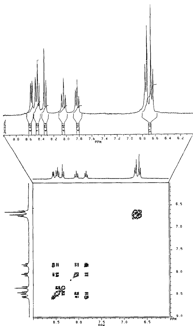
Fig. 1. 250 MHz COSY ^1\text{H} NMR spectrum of [\text{ReO}(\text{SC}_6\text{H}_4\text{Me-}p)_2(\text{terpy})]\text{ReO}_4 in acetone- d_6 over the aromatic region (6.0–9.0 ppm).
