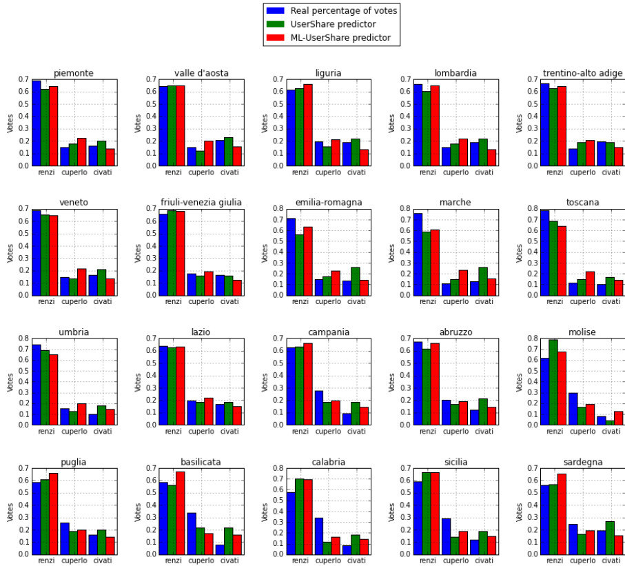
Fig. 4. Regional predictions and actual voting results.
