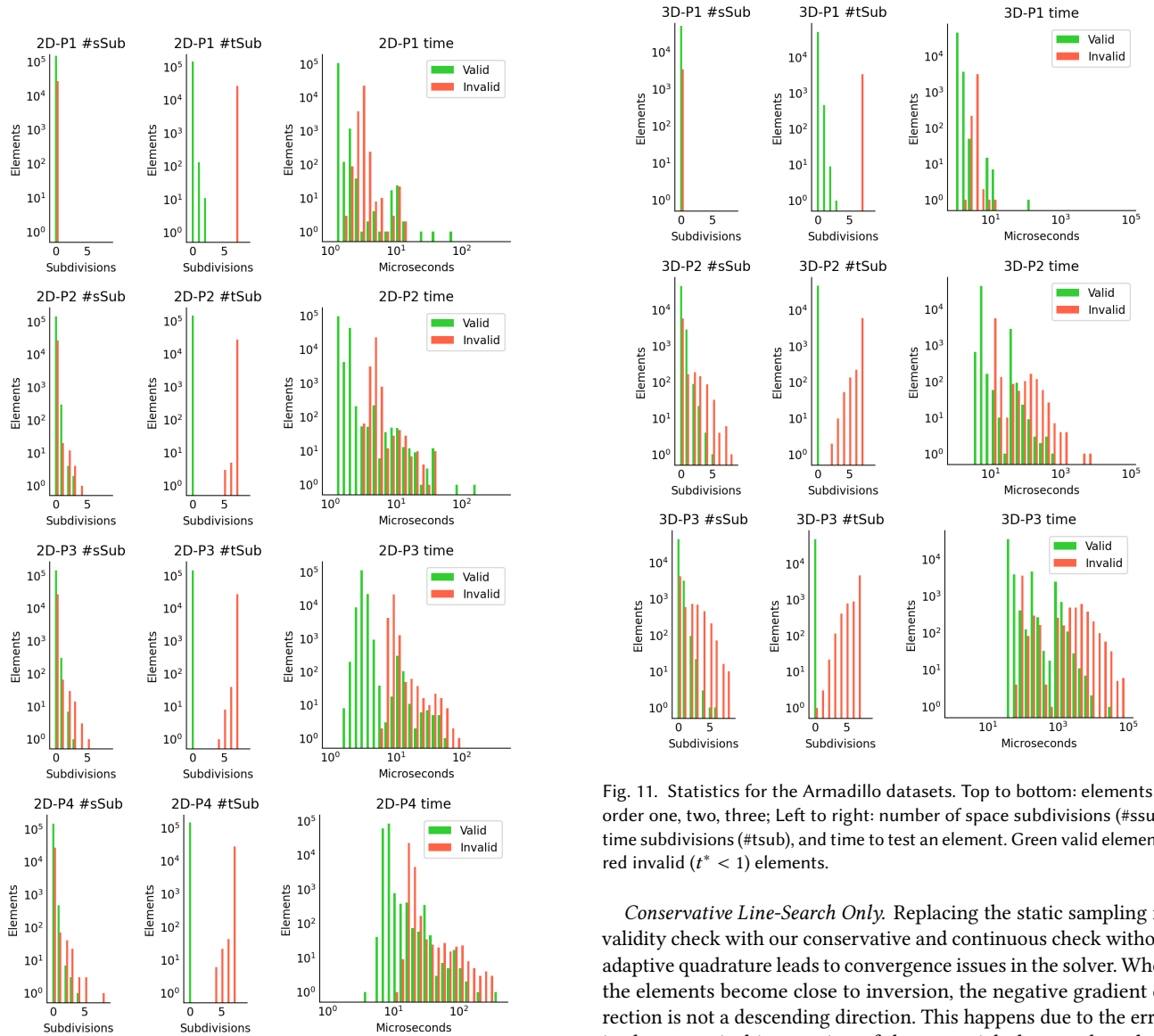
Fig. 10. Statistics for the Kangaroo datasets. Top to bottom: elements of order one, two, three, four; Left to right: number of space subdivisions (#sSub), time subdivisions (#tSub), and time to test an element. Green valid elements; red invalid ( t^* < 1 ) elements.
