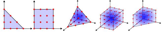
Fig. 5. Reference elements with domain points of order three: triangle, square, tetrahedron, hexahedron, prism.
