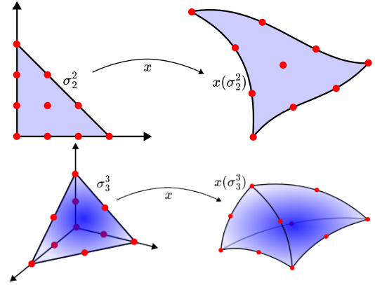
Fig. 6. Above: A domain \sigma_2^2 with its domain points of order three and the geometric map x to the physical element x(\sigma_2^2) with Lagrange control points. Below: likewise for an element \sigma_3^3 of order two.
