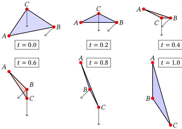
Fig. 3. A dynamic linear element with linear trajectories that flips twice in a time interval, resulting in an element, that is, valid at both time steps, but invalid in the transition. Assuming point A remains fixed, the arrows represent the velocities of points B and C to reach the final position. The color of each element indicates the sign of the determinant at time t : blue if positive and red if negative. The dynamic element's Jacobian determinant is a univariate polynomial in t of degree 2, with two distinct roots in [0, 1] .
