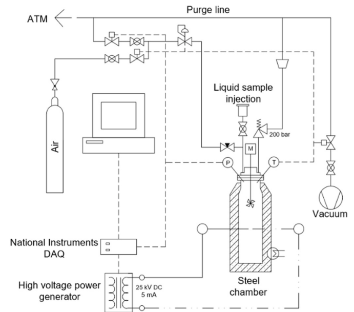
Fig. 1. Schematic representation of the experimental setup used in this study for explosion tests.
