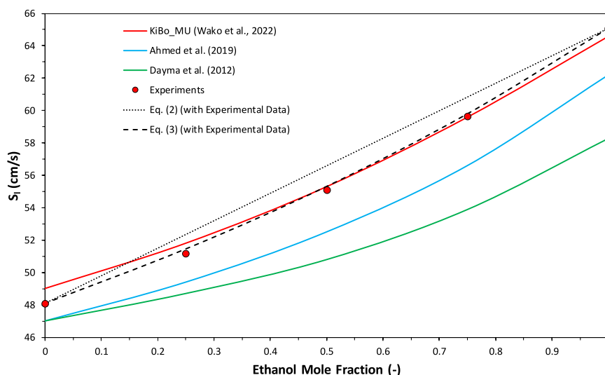
Fig. 5. Laminar burning velocity, S_L , versus ethanol mole fraction in the fuel (ethanol-ethyl acetate) mixture as obtained from closed vessel explosion experiments (mean values represented by circles) and computed using different chemical kinetic mechanisms (solid lines) ( \phi = 1.1 ). The dotted and dashed lines correspond to the predictions calculated using Eq. (2) and Eq. (3), respectively, with the experimental data of ethanol and ethyl acetate.
