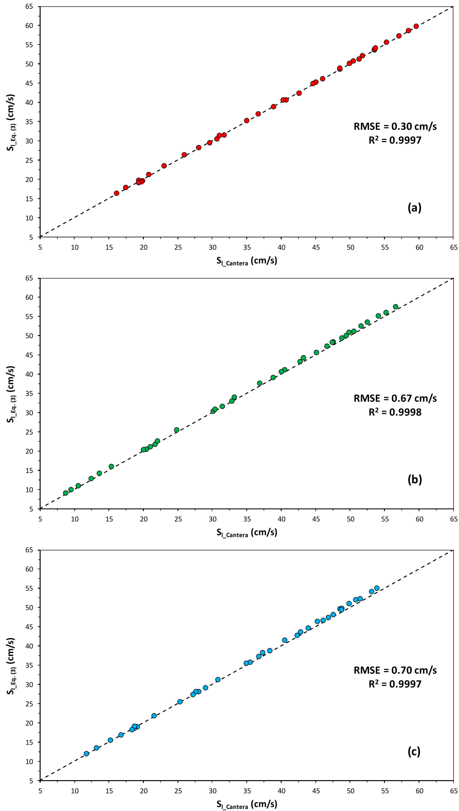
Fig. 6. Laminar burning velocity of ethanol-ethyl acetate/air mixtures predicted using Eq. (3), S_{L\_Eq.(3)} , as a function of the corresponding laminar burning velocity computed using the Cantera software, S_{L\_Cantera} , with the three different detailed chemical kinetic mechanisms developed, respectively, by (a) the University of Bologna (Wako et al., 2022), (b) Ahmed et al. (2019), and (c) Dayma et al. (2012). All values of equivalence ratio (0.6-1.7) and ethanol mole fraction in the fuel mixture (0.25, 0.50, and 0.75) were considered. For each mechanism, the root mean square error, RMSE, and the coefficient of determination, R^2 , are also reported.
