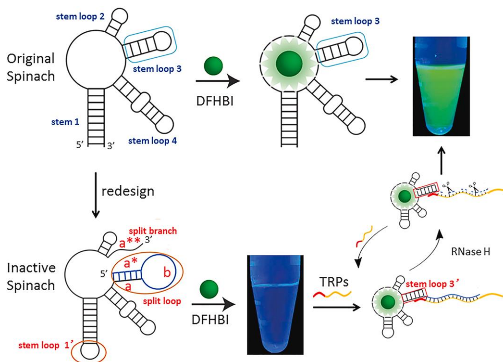
Figure 5. Principle of the telomerase reaction product-initiated Spinach reconstruction. Reprinted with permission from [45] Copyright (2022) Elsevier.
