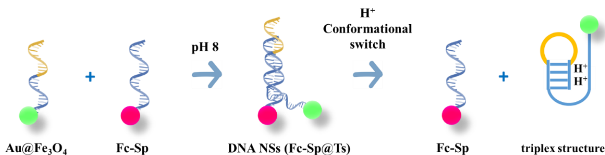
Figure 2. Schematic diagram of the conformational switch of pH-responsive DNA nanostructures (DNA NSs, Fc-Sp@Ts) induced by hydrogen ion ( H^+ ) released from PTP1-based LAMP reactions initiated by the primers with the help of dNTPs and Bst polymerase, liberating the signal probe labeled with electroactive ferrocene (Fc-Sp). Readapted from [9].
