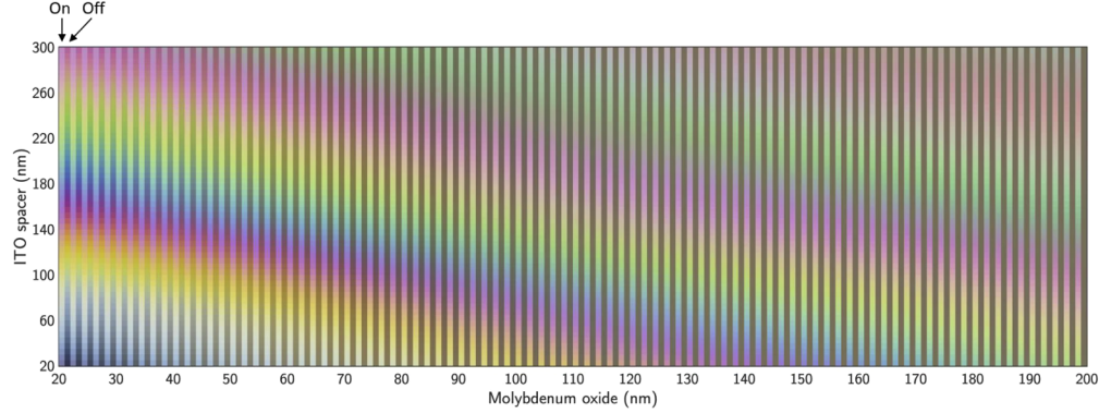
Fig. 3. Simulation of colors than can be achieved with the designed reflective display ITO/MoO x /ITO/Pt (normal incidence and non polarized light) for MoO x thicknesses from 20 to 200 nm and ITO spacer thicknesses from 20 to 300 nm. Each MoO x thickness point shows the reflected color for x = 2.9 (left) and for x = 2.1 (right) case. For x=2.9 ( on mode) a colored line can be observed whose color changes as a function of the ITO spacer thickness. For x=2.1 ( off mode) a uniform line can be seen since there is no dominant color due to the high absorptivity in the active layer. This pale color is more notorious as the MoO x thickness is increased.
