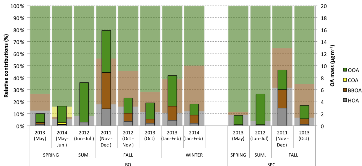
Figure 5. Organic aerosol source contributions for each site and each Supersito campaign. Relative contributions are shown as shaded histograms (referring to the left axis) in the background of the absolute ones (referring to the right axis).
