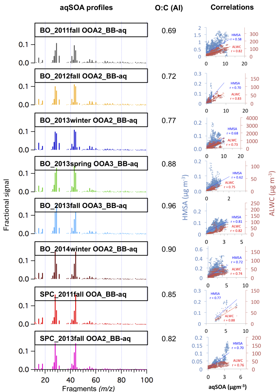
Figure 9. OOAx_BB-aq main features: the left column shows the mass spectral profile of each BB-aqSOA component identified during the Supersito campaigns; the OOA factors are numerically ordered for each campaign based on their O : C ratios; the central column shows the O : C elemental ratios of the same factors; the right column illustrates the correlation between their concentration time series and the HMSA (in blue) and the ALWC (in red).
