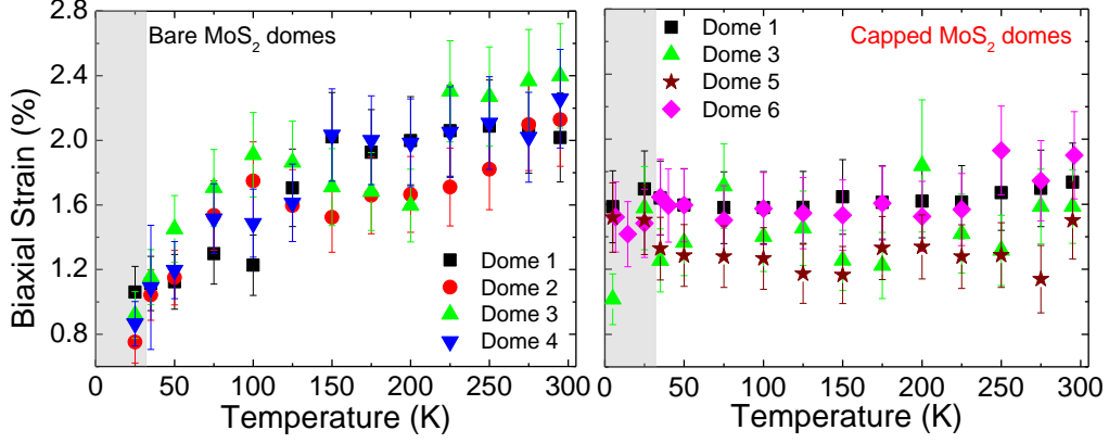
Figure S2. Bi-axial strain vs temperature calculated from the Raman shifts of the E_{2g} peak (in-plane mode of oscillation) of several MoS 2 domes. The value of strain is calculated using the equation
