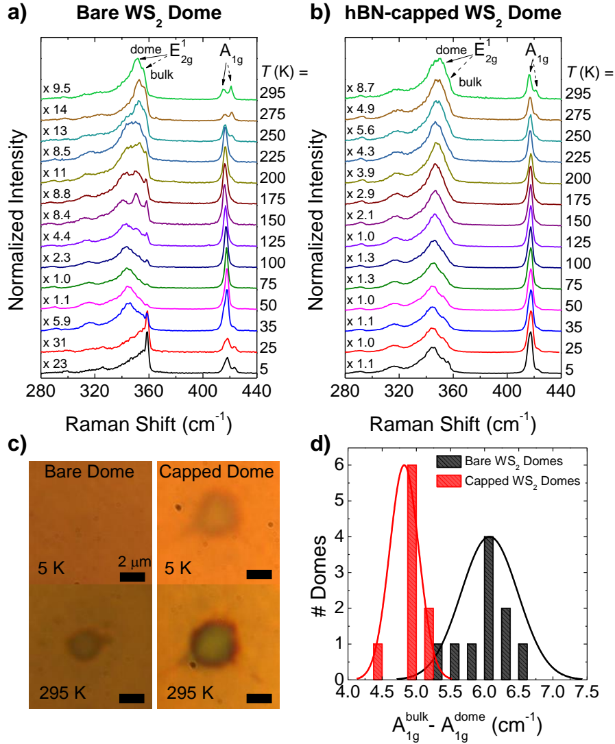
Figure S3. Raman study of bare and hBN-capped WS 2 domes. a)-b) Stacked \mu -Raman spectra at different temperatures of a bare a) and hBN-capped b) WS 2 dome. The laser excitation wavelength is equal to 532 nm and the laser power is equal to 30 \mu W. The peaks refer to the E_{2g}^1 (in-plane) and A_{1g} (out-of-plane) modes of oscillation associated to the bulk crystal (dashed arrow) and to the dome membrane (full arrow). Next to each spectrum an intensity factor indicates the ratio between the maximum intensity of the corresponding set of spectra and the intensity for that specific temperature. While the bare WS 2 dome's spectra show an erratic behaviour both in lineshape and in intensity, the regularity of the capped dome's spectra, on the other hand, reflects the conservative effect of hBN. c) Optical images of the domes of panel a) (left column) and panel b) (right column) at temperatures of 5 K and 295 K. The deflation, at low T , undergone by the bare dome is in contrast with the minimal changes in volume experienced by the hBN-capped dome. Scalebar, 2 \mu m. d) Histogram collecting the differences in Raman shift, at RT, between the peak associated to the bulk A_{1g} mode of oscillation and the one associated to the dome membrane. The peak values were extracted with Lorentzian fits performed on the spectra of several bare (black bars) and hBN-capped (red bars) WS 2 domes. Since strain is responsible for the softening of the Raman mode, the reduction from a mean
