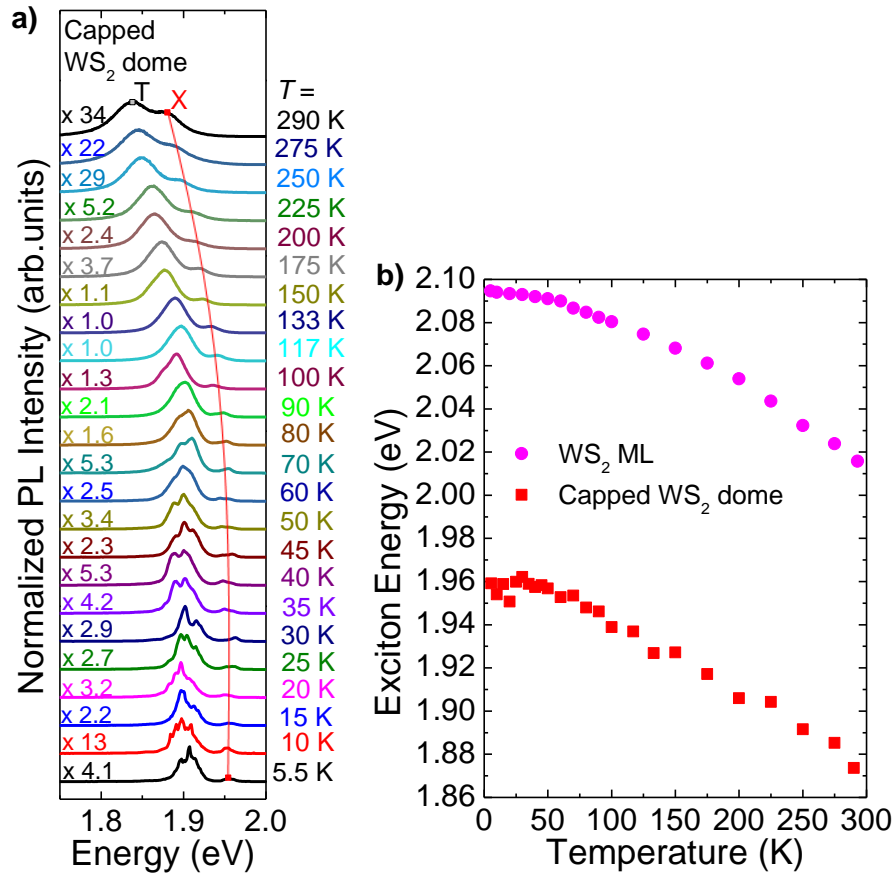
Figure S5. a) \mu -photoluminescence (PL) of a WS 2 dome capped with few-layer hBN as a function of temperature. Excitation wavelength equal to 532 nm and laser power equal to 4.4 \mu W. The exciton peak (X) is highlighted at 290 K and 5.5 K by a red square, with its evolution at intermediate temperatures followed by a red line as a guide for the eye. The predominant energy band at lower energy (labeled T) is likely due to charged exciton recombination. [5,6] The intensity factors next to each spectrum are the ratio between the maximum PL intensity at 117 K and the one of the corresponding spectrum. b) Energy of exciton X vs temperature extracted from the spectra of panel a) via Voigt fits (red squares) compared with the evolution in energy of the exciton peak of an unstrained WS 2 ML deposited on SiO 2 (magenta circles). Apart from a rigid shift caused by tensile strain, the two trends are almost identical, confirming the preserving effect of hBN on the dome geometry and strained configuration.
