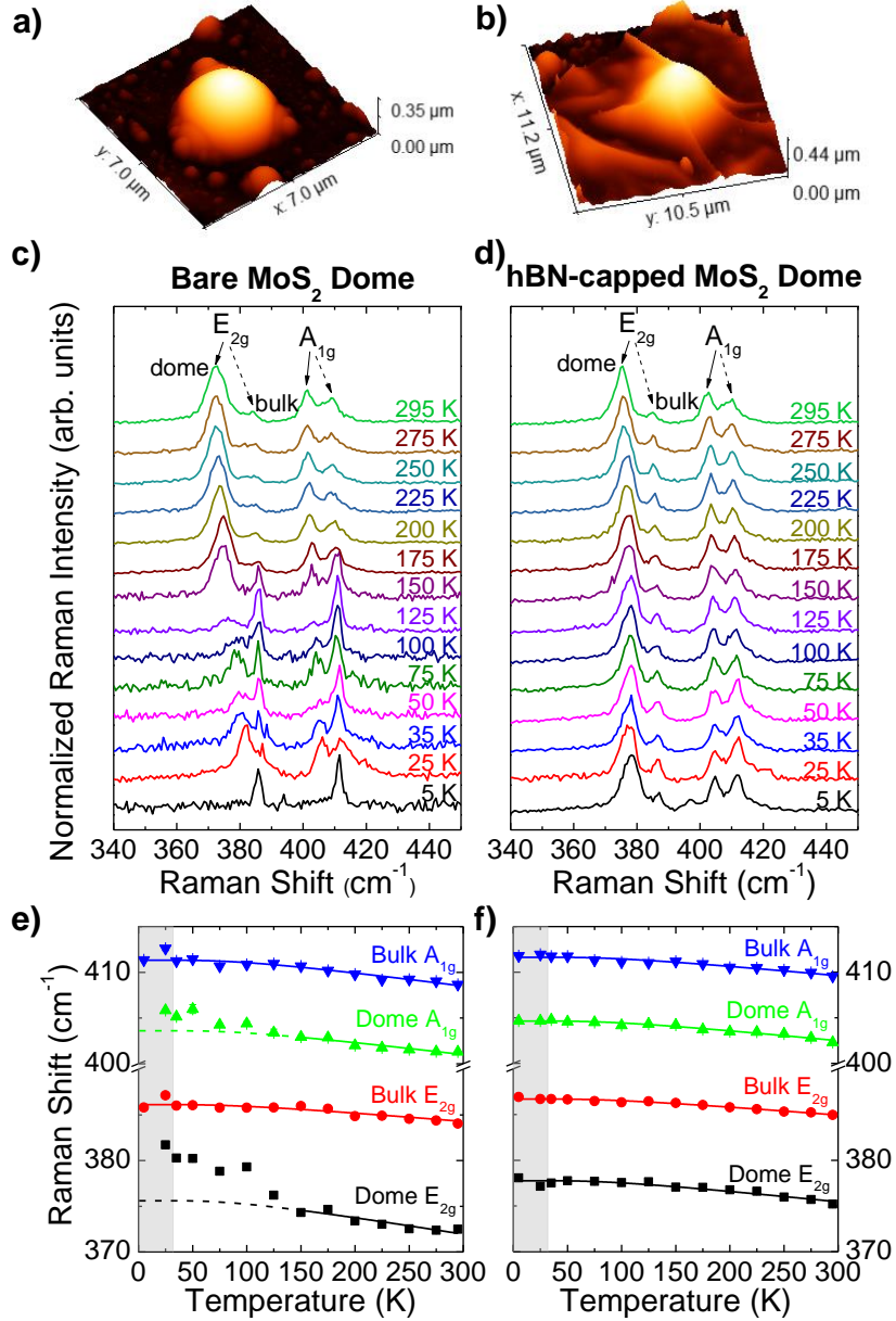
Figure S1. Temperature-dependent \mu -Raman studies of a MoS 2 dome before and after capping with few-layer hBN. a)-b) AFM 3D maps of the dome before a) and after b) the capping procedure. c)-d) Stacked \mu -Raman spectra for all the temperatures considered of the MoS 2 dome before and after hBN capping (laser excitation wavelength equal to 532 nm and laser power equal to 30 \mu W.). The peaks refer to the E 2g (in-plane) and A 1g (out-of-plane) modes of oscillation associated to the bulk crystal (dashed arrow) and to the dome membrane (full arrow). e)-f) Evolution with temperature of the peaks of panels c) and d) extracted by performing Lorentzian fits of the \mu -Raman spectra of the bare and capped dome. The trends are fitted with \omega(T) = \omega_0 + A \left[ 1 + 2 / \left( e^{\frac{\hbar\omega_0}{2k_B T}} - 1 \right) \right] , where only the lower-order three-phonon processes of the anharmonic Klemens model are taken into account via the parameter A. [1,2] The almost
