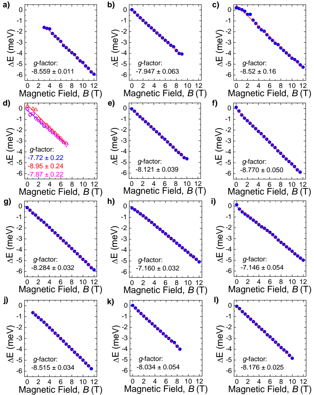
Supporting Figure 6. g -factor of \text{WS}_2 quantum emitters.
