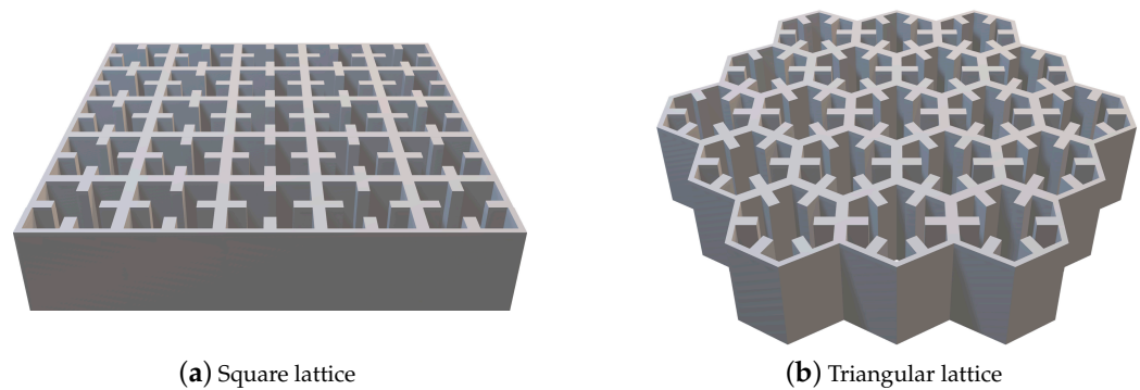
Figure 1. Open-ended ridged waveguide elements in square and triangular lattices.
