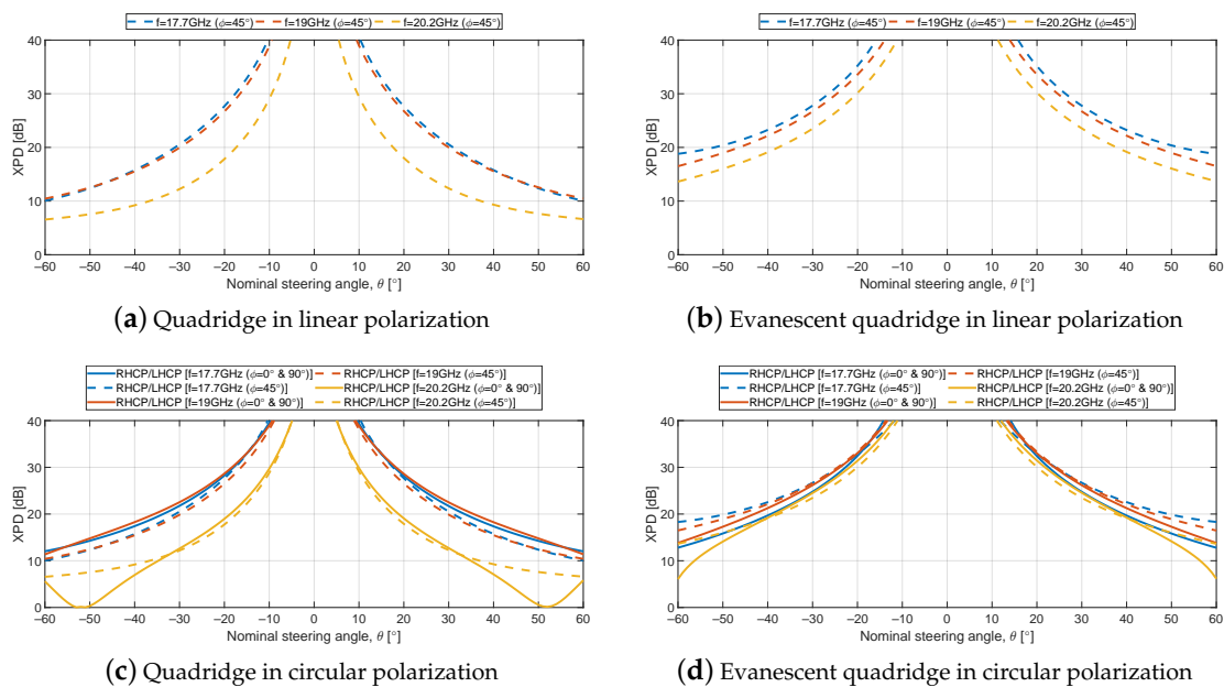
Figure 14. XPD for both quadridge designs.
