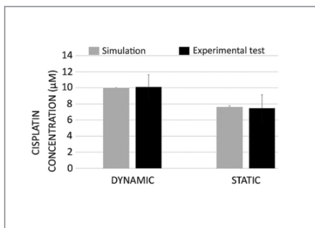
Fig. 6: Concentration of cisplatin in OCM after 7 days culture in dynamic or static conditions
