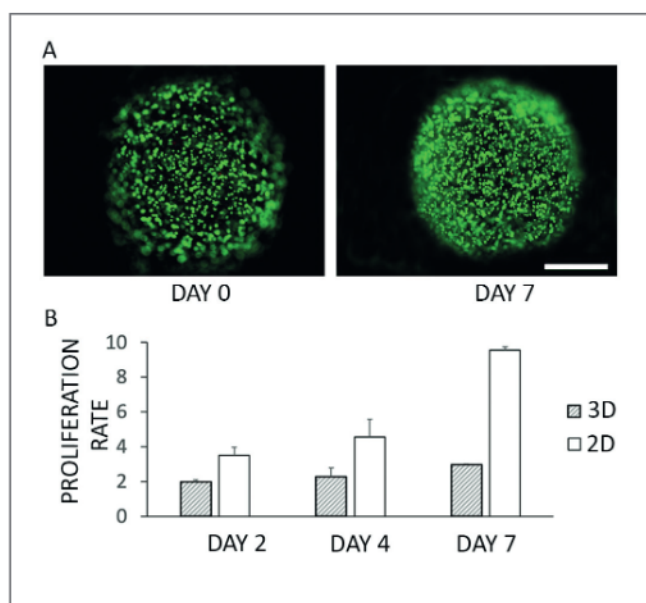
Fig. 2: Cell viability and proliferation of OCM in culture (A) Cell viability represented by live/dead images of OCM after 4 hours (Day 0) and 7 days (Day 7) of culture. Scale bar is 500 \mu\text{m} . (B) Quantitative analysis of the proliferation rate of ovarian cancer cells embedded within alginate hydrogels (3D) or cultured in monolayers (2D) assessed by Alamar Blue assay. Values are reported as mean \pm SD. (N = 3 biological replicates; n = 2 technical replicates).
