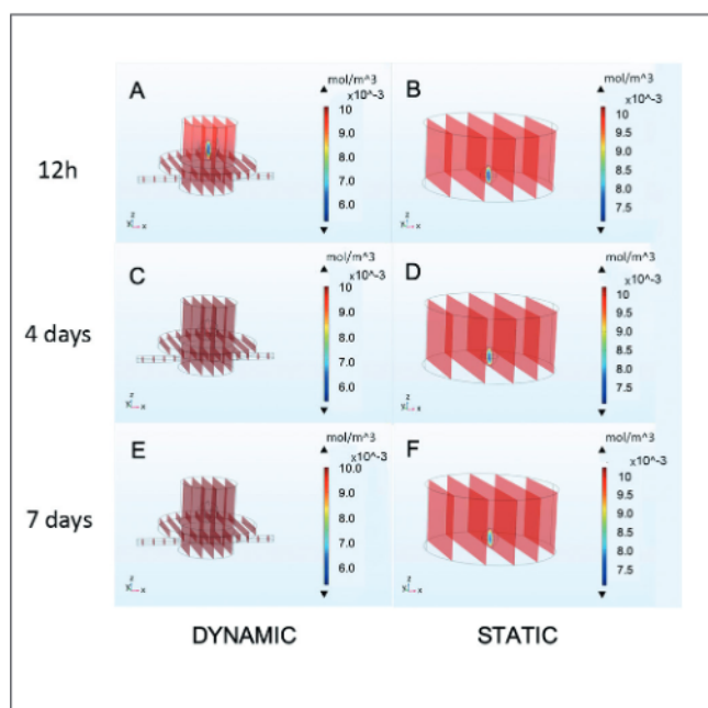
Fig. 5: Distribution of cisplatin in dynamic and static conditions at 10 \mu M and different time points (A) dynamic; 12 h, (B) static; 12 h, (C) dynamic; 4 days, (D) static; 4 days, (E) dynamic; 7 days, (F) static; 7 days. While the dynamic condition shows a complete drug distribution within the 3D volume after 7 days of culture, a strong gradient is still present under static conditions.
