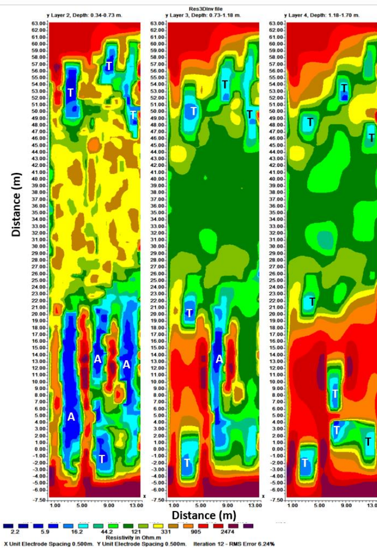
Fig. 3. EM data: resistivity distribution at several depths.
