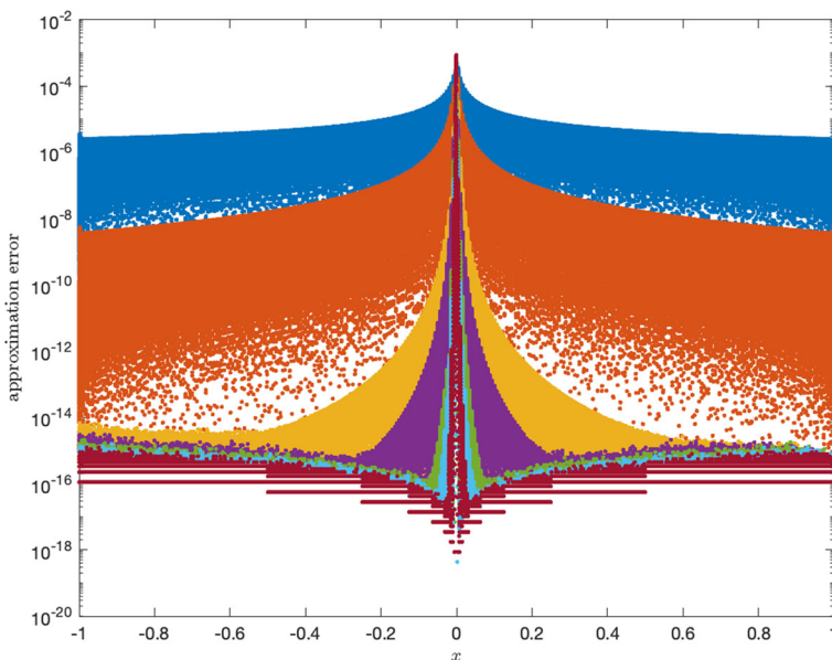
Fig. 3 Pointwise absolute error when interpolating the function f(x) = |x| with d = 1 , h^* = 1.0e-3 and h = 5h^* for increasing values of \gamma = 1, 2, \dots, 7 . The error is plotted in blue for \gamma = 1 , in red for \gamma = 2 and so on
