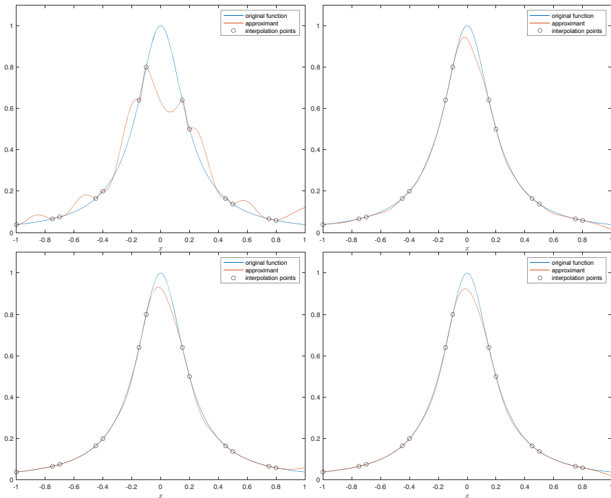
Fig. 1 The rational interpolant \tilde{r}(f, x) of the Runge function f(x) = 1/(1+25x^2) on the interval [-1, +1] , for \gamma = 2 , h/h^* = 5 , h^* = 0.05 and d = 0, 1, 2, 3 (from left to right and top to bottom)
