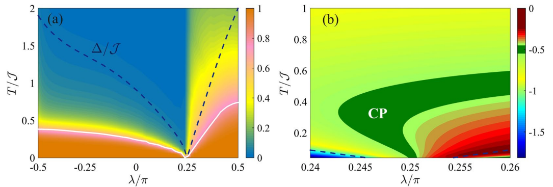
Figure 9. Phase diagram of the Kitaev chain with long-range pairing. (a) QFI normalized to its low-temperature value, F_Q[|\hat{\rho}_T\rangle]/F_Q[|\psi_0\rangle] (color scale), in the \lambda - T phase diagram. (b) Scaling coefficient \beta = d \log F_Q[|\hat{\rho}_T\rangle]/d \log T . In both panels the white line is T_{\text{cross}} and the blue dashed line is the energy gap \Delta . Here N = 50 and \alpha = 0 .
